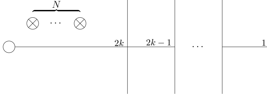
Figure 3.4: Magnetic brane system for the tensor branch of the D_N^{5u2k}([1^{2k}]) SCFT.
