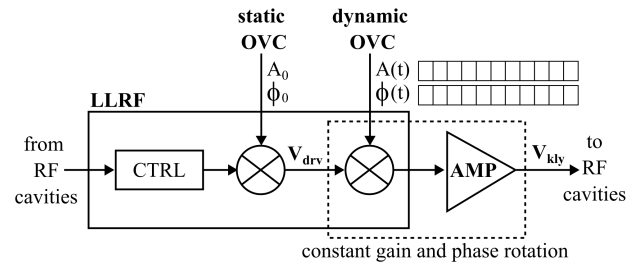
Figure 3: The dynamic output vector correction ensures that the combined effect of the LLRF drive modulation and the high power amplifier results in a constant input-output gain and phase rotation.
