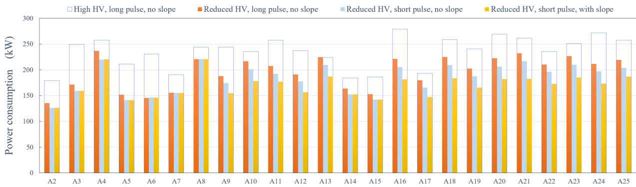
Figure 5: Energy savings across all modulators of the EuXFEL linacs, showing the benefits of the three successive approaches.
