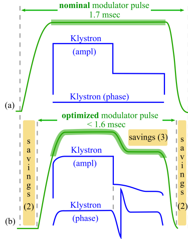
Figure 2: Schematic representation of the modulator pulse (green) scheduled around the RF pulse (blue), for the unmodified case (a) and for the shorter modulator pulse including a step down during the beam time (b). If left uncorrected, the resulting change in gain and phase of the klystron output signal over the course of the RF pulse make field regulation extremely challenging.
