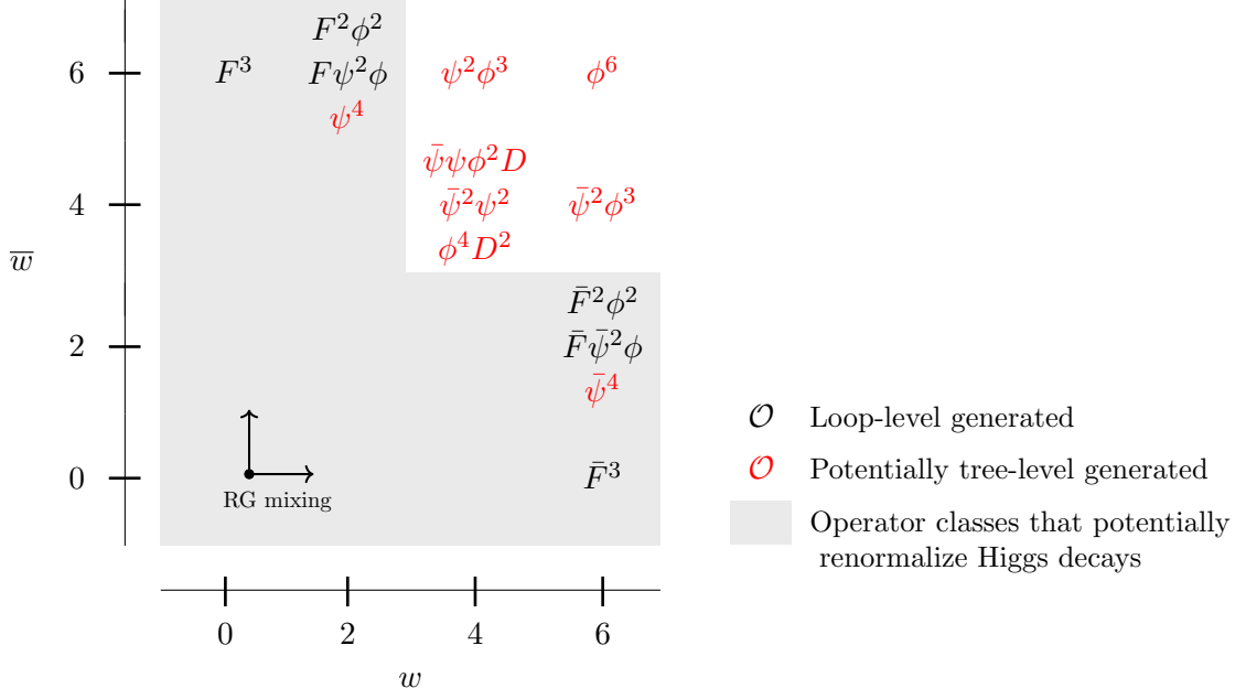
Figure 1: Operator classes in the Warsaw basis of the SMEFT at dimension six, distributed according to their holomorphic weights. Following Ref. [43], the arrows indicate the direction in which one-loop RG mixing is possible. That is, operators do not mix into other operators that are on their left or below them in the diagram. The operators in red can be tree-level generated, while LLOs are written in black. The shaded area contains all operator classes which could potentially mix into the Higgs decays, captured by the operator classes F^2\phi^2 and \bar{F}^2\phi^2 .
