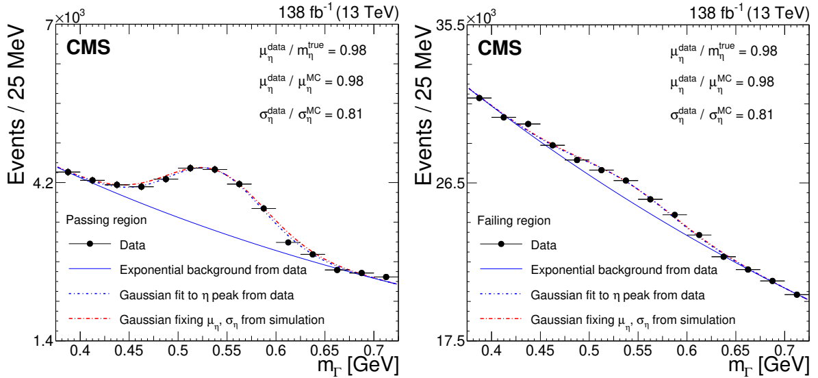
Figure 1: Cluster mass ( m_\Gamma ) distribution in data for both the passing (left) and failing (right) regions, in the energy range for which the \eta meson is expected to form a single \Gamma candidate. The signal (background) is modeled by a Gaussian (exponential) function. Blue and red dashed lines depict Gaussian fits to the data and Monte Carlo (MC) simulation, respectively. The solid blue line shows the background component of the fit. Ratios of the Gaussian fit means ( \mu ) and widths ( \sigma ) are displayed, where m_\eta^{\text{true}} is the true mass of the \eta meson.
