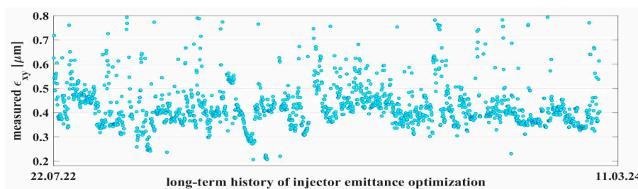
Figure 2: Long-term measurement history of transverse projected emittance of the electron bunch in the injector at 250 pC.
