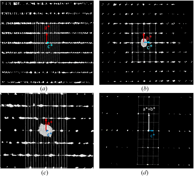
Figure 4 Images of the reconstructed reciprocal space. (a) The projection of the reciprocal space of Cr3_HH266 viewed down [010] showing the unit cell of the 6R polytype with the threefold superstructure along c^* . (b) The [010] projection of Cr2_HH266 with much less additional reflections along c^* compared to (a). The reciprocal unit cell corresponds to the nolanite-type phase. (c) h0hl reflections of Cr3_HH266, i.e. a single slice of the reciprocal space, cut out of the projection in (a). In comparison to Cr2_HH266 additional streaks are visible. (d) hh2hl reflections of Cr2_HH266. The systematic extinctions of the c -glide plane are slightly violated due to additional reflections from the rhombohedral phase. The grid represents the projection of the reciprocal unit cell onto the image plane.
