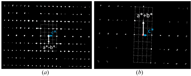
Figure 3 Slices of the reconstructed reciprocal space of the \text{SnGe}_4\text{N}_4\text{O}_4 phase of Cr1_HH228. (a) Viewing direction [110] showing the hh0l reflections. For 000l reflections, l = 2n is clearly visible, no other extinctions are visible. (b) Viewing direction [110] showing the hh2hl reflections, l = 2n is only violated by weak reflections. The grid shown in the figures represents the corresponding projections of the reciprocal unit cell onto the image plane. As \mathbf{a}^* and \mathbf{b}^* are not parallel to this plane in the given viewing directions, the grid points representing the projection of \mathbf{a}^* or \mathbf{b}^* onto the image plane are not occupied by reflections in the zero layer of the reciprocal space, however in higher layers above and below.
