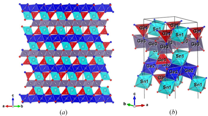
Figure 8 Structure of the rhombohedral phase, space group R\bar{3}m . Color code is the same as for the nolanite-type. Now there are two different non-equivalent O-layers formed by octahedra centered by Ge2 (shown in blue) and Ge3 (shown in gray). (a) Projection of the unit cell along [110], visualizing the polyhedron layers. (b) A part of the unit cell in perspective view, highlighting the connections between the different cation polyhedra in more detail.
