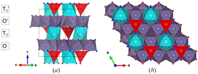
Figure 7 Structure of the nolanite-type phase viewed perpendicular to the c -axis ( a ) and along the c -axis ( b ). Ge1 tetrahedra are shown in red and Sn octahedra are shown in turquoise.
