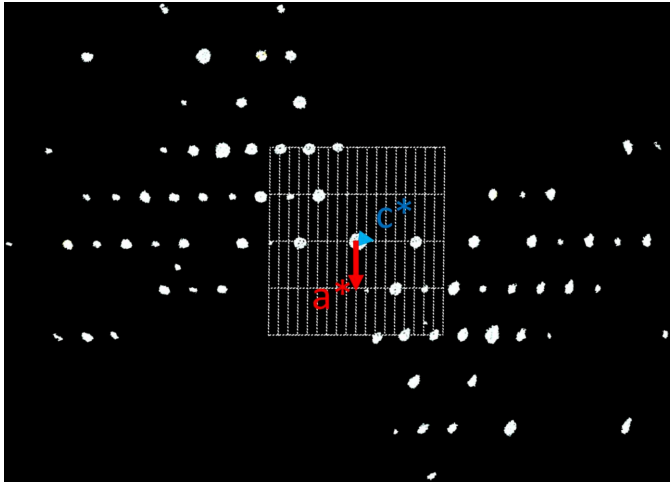
Figure 5 Reciprocal space of Cr4_HH266. Slice of the h\bar{1}0l reflections, showing the presence of an obverse rhombohedral centering with hki l: -h+k+l = 3n . The l = 2n condition for h\bar{1}0l reflections indicating a c -glide plane is violated giving R-- as an extinction symbol.
