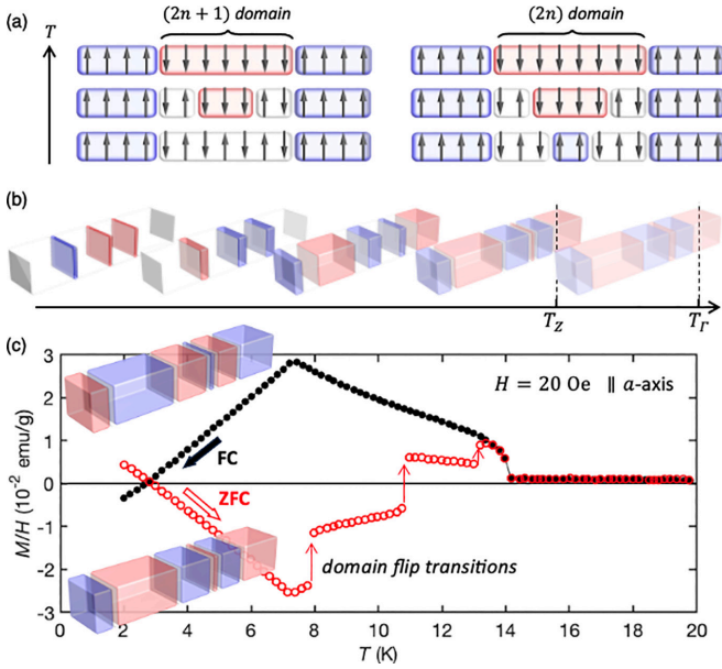
FIG. 4. (a) Illustration of the magnetic phase separation scenario below T_Z . Each layer of \text{Eu}_5\text{In}_2\text{Sb}_6 is represented by an arrow indicating the direction of the Ising (per-layer) net magnetic moment. Up (down) domains of the \mathbf{q}_T state are colored blue (red). Interfaces between \Gamma domains may provide natural nucleation points of the Z state (white). \Gamma domains with an even ( 2n ) number of layers prevent the formation of a homogeneous Z ordered state. They leave behind antiferromagnetic domain walls that carry a net magnetic moment and could also contribute to hysteretic effects. (b) Sketch of the thermal evolution of an \text{Eu}_5\text{In}_2\text{Sb}_6 slab, colored in analogy to (a). (c) Field-cooled and zero-field cooled (FC/ZFC) curves of the magnetic susceptibility measured with a weak (20 Oe) bias field along the a axis. Magnetization reversal and domain flip transitions [indicated by inset illustrations] provide a tentative explanation for these unusual characteristics.
