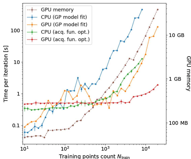
FIG. 26. Performance scaling with dataset size for BoTorch/GPyTorch (0.9.4/1.11) libraries on a single-objective optimization run. Synthetic five-variable quadratic objective was used with Monte Carlo version of UCB acquisition function and 100 Adam optimizer iterations. GPU memory usage is only applicable to GPU runs.
