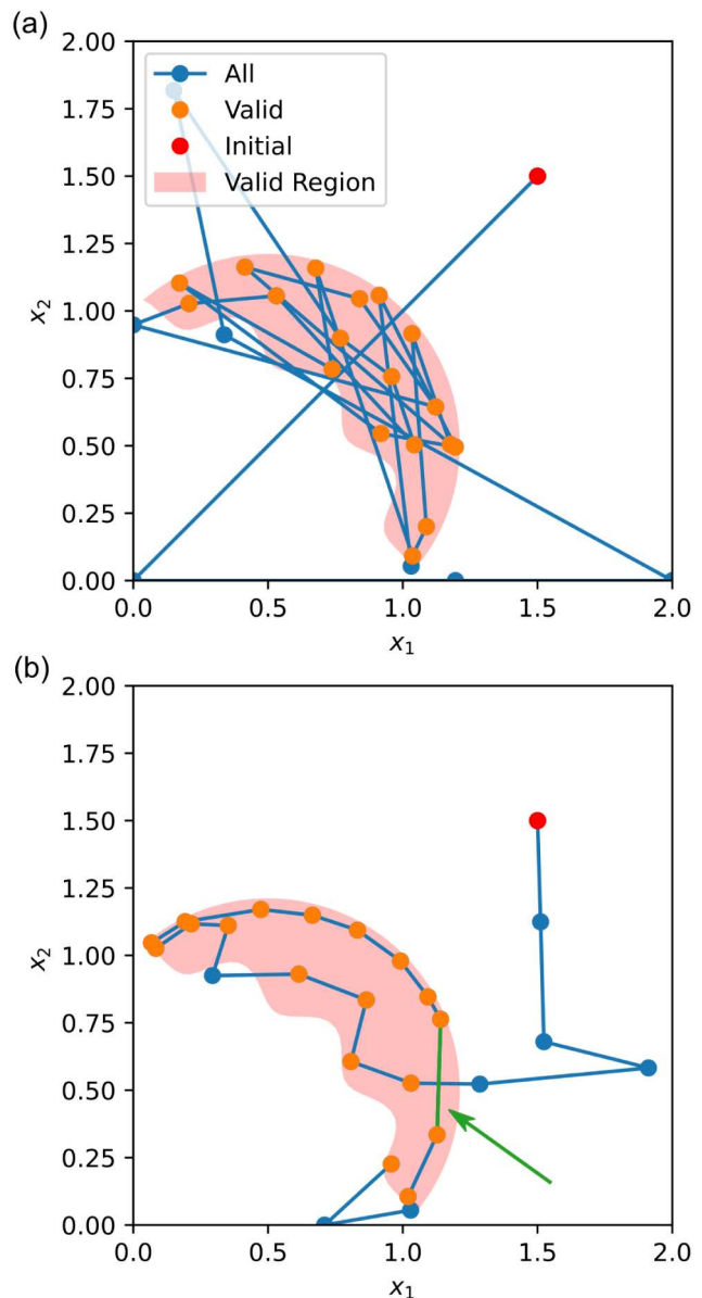
FIG. 20. Demonstration of proximal biasing effects during Bayesian exploration (BE) of the constrained TNK test problem. (a) Normal BE. (b) BE using proximal biasing with l = 0.1 . The green arrow highlights a step where a larger jump in parameter space was allowed by proximal biasing. Reproduced from [86].
