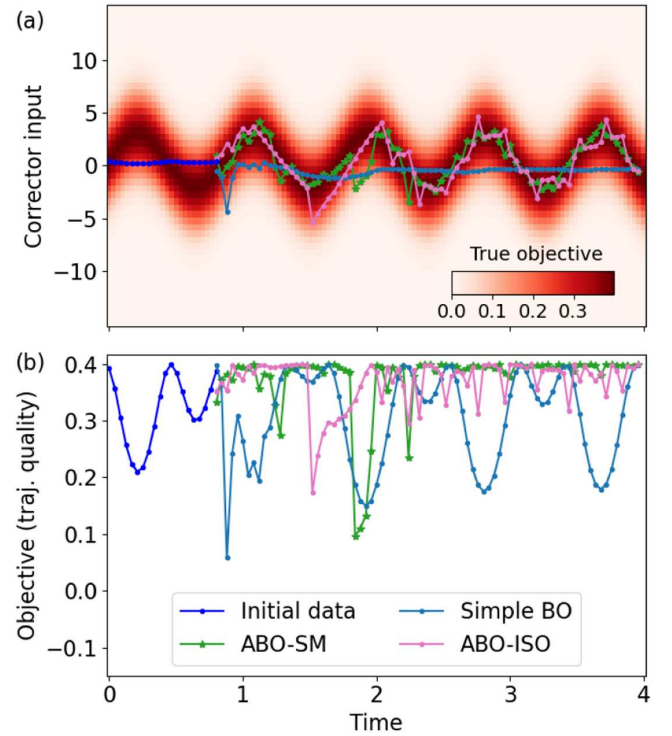
FIG. 12. Simulated application of standard and time-aware BO in a drifting trajectory stabilization problem. Simple BO settles on the mean value of the oscillations. ABO-ISO (isotropic) follows the changes but lags them because it only uses isotropic (local) kernel. ABO-SM (spectral mixture) captures long-range correlations and eventually correctly predicts necessary future changes in phase. By default, ABO-SM continues to explore around maximum value for optimization, producing a small step jitter. It can be eliminated by using the posterior mean as the acquisition function at the cost of convergence speed.
