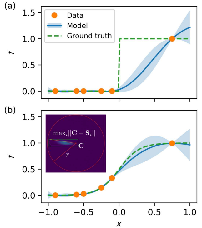
FIG. 24. Comparison between GP modeling of hard and soft constraining functions. (a) GP modeling of a heaviside constraining function does not accurately predict constraint values due to a single sharp feature that cannot be learned without dense sampling on either side of the constraint boundary. (b) Smooth constraining functions with a single characteristic length scale are more accurately modeled with GP modeling. Inset: Visualization of bounding box constraint function f(x) = \max_i \{||\mathbf{C} - \mathbf{S}_i(x)||\} used to keep beam distributions inside an ROI, where r is the radius of a circular ROI, \mathbf{C} is the center coordinates of the ROI, and \mathbf{S}_i are corner coordinates of a bounding box around the beam.
