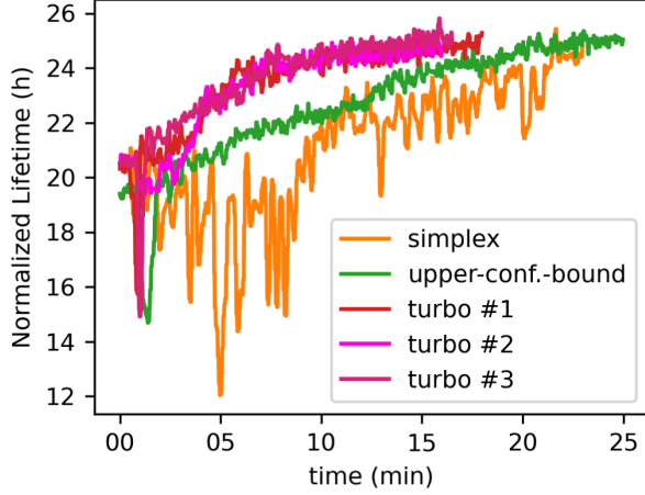
FIG. 22. Trust region BO (TuRBO), simplex, and UCB applied to the minimization of total losses (maximization of lifetime) at the ESRF-EBS storage ring. Adapted from [96].
