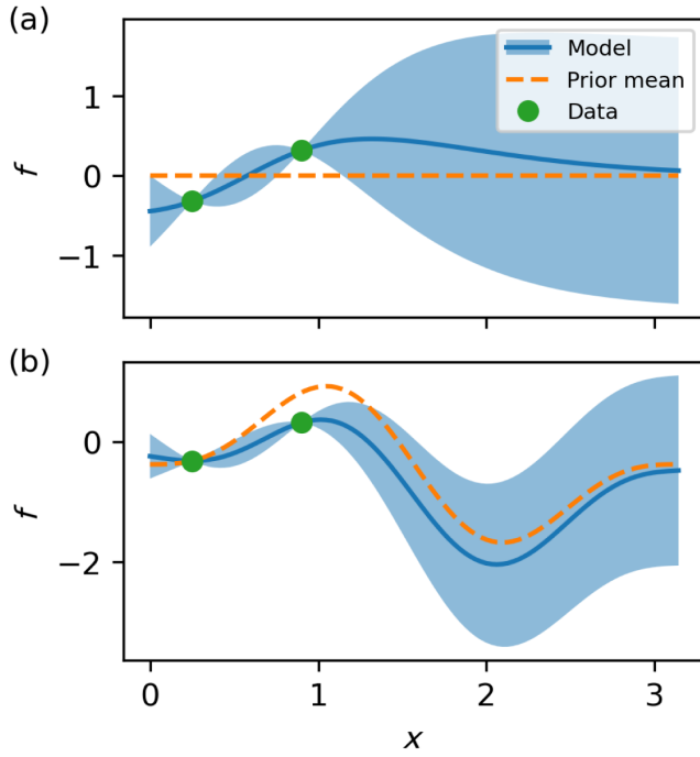
FIG. 9. Illustration of nonzero prior mean. In the absence of local data, the mean of the posterior distributions reverts to (a) zero or (b) the nonzero prior mean. The variance remains unchanged.
