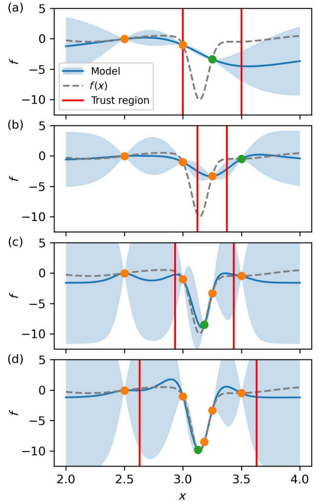
FIG. 21. One-dimensional visualization of trust region BO (TuRBO) applied to a minimization problem with the UCB acquisition function. (a)–(d) Sequential evolution of the GP model and sampling pattern. Orange circles denote objective function measurements and green circles denote the most recent sequential measurement at each step.
