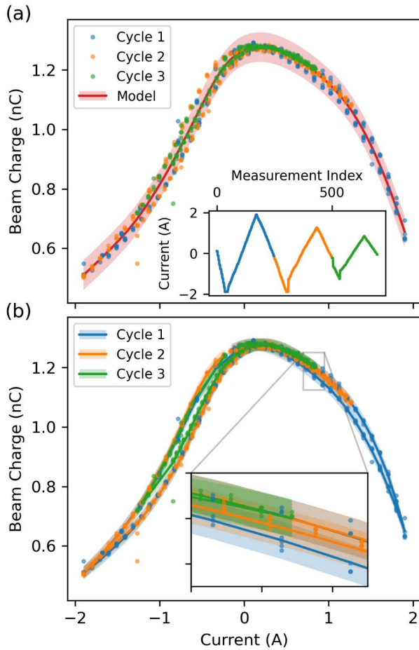
FIG. 14. Demonstration of combining GP models with a differentiable physics model of magnetic hysteresis. (a) Measured beam charge after passing through an aperture in the APS injector is plotted over three cycles of varying the current in an upstream quadrupole. Transmitted beam charge measurements are not repeatable due to hysteresis effects in the upstream quadrupole. (b) GP modeling with differentiable hysteresis model included accurately predicts beam charge over multiple hysteresis cycles with improved (reduced) uncertainty predictions. Reproduced from [28].
