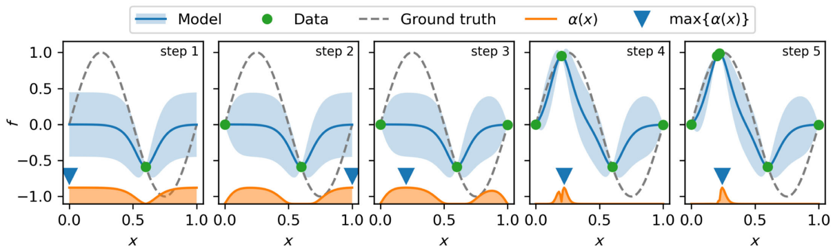
FIG. 3. Illustration of the Bayesian optimization process to find the maximum of a simple function. A Gaussian process (GP) model makes predictions of the function value (solid blue line) along with associated uncertainties (blue shading) based on previously collected data. An acquisition function then uses the GP model to predict the “value” of making potential future measurements, balancing both exploration and exploitation. The next observation is chosen by maximizing the acquisition function in parameter space. This process is repeated iteratively until optimization goals have been reached.
