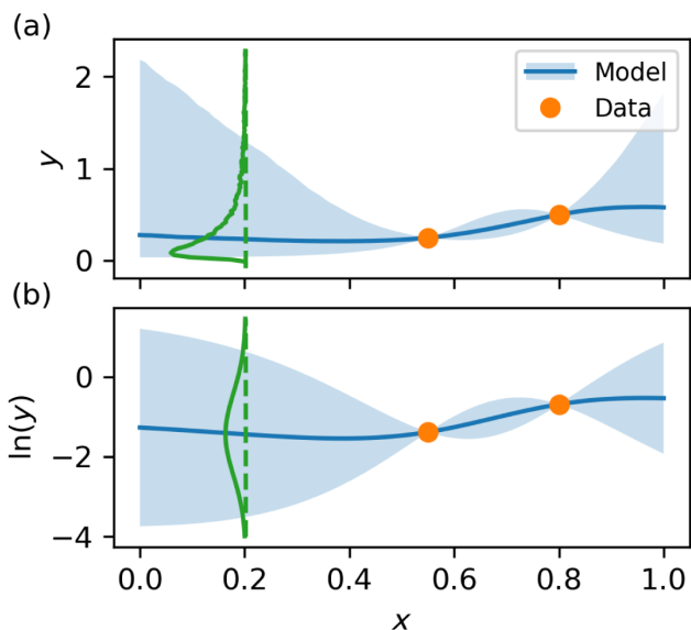
FIG. 11. Example of using log transformations in GP modeling for strictly positive output values. Data in real space (a) are transformed to log space before fitting a GP model (b). Samples drawn from the GP model in log space can then be transformed back into real space to make GP predictions. The resulting likelihood in real space is then a log-normal distribution which is strictly positive.
