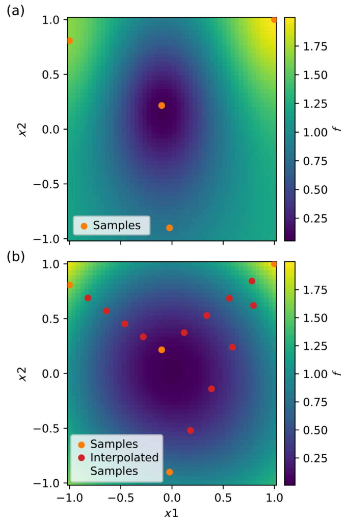
FIG. 25. Comparison between GP modeling of the two-dimensional sphere function f(x_1, x_2) = x_1^2 + x_2^2 with and without interpolated measurements. (a) Shows the posterior mean of the GP model with four measurements taken sequentially. (b) Shows the same four measurements taken sequentially but with interpolated points in between each measurement. Incorporating interpolated points in the dataset leads to higher modeling accuracy, leading to accurate identification of the sphere function minimum at the origin.
