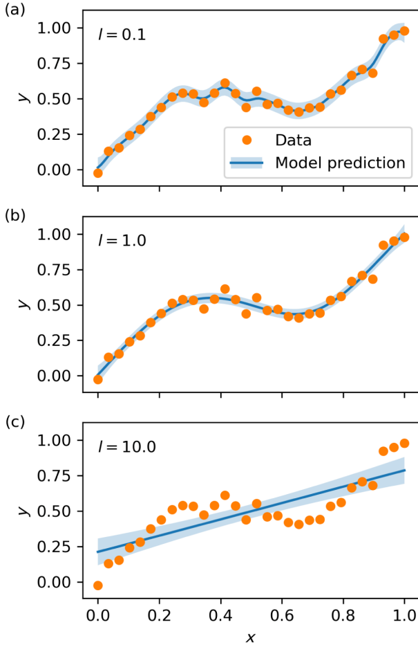
FIG. 6. Visualization of how the length scale hyperparameter l effects GP modeling. Three GP models are trained on the same dataset using a Matérn kernel with fixed length scales of (a) 0.1, (b) 1, and (c) 10. Remaining hyperparameters are trained by maximizing the marginal log-likelihood.
