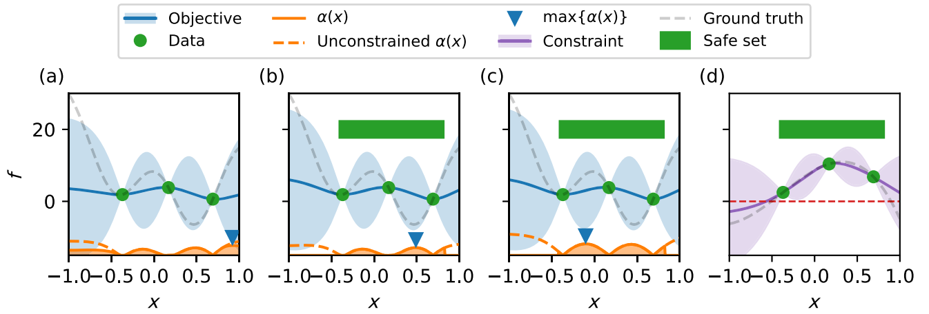
FIG. 17. Comparison between different constrained Bayesian optimization algorithms. (a) Weighting the acquisition function by the probability of satisfying the constraining function [73]. (b) Acquisition function optimization within a safe set using MoSaOpt in exploitation mode [32] and (c) SafeOpt [75]. (d) The constraint function, where valid regions satisfy c(x) > 0 .
