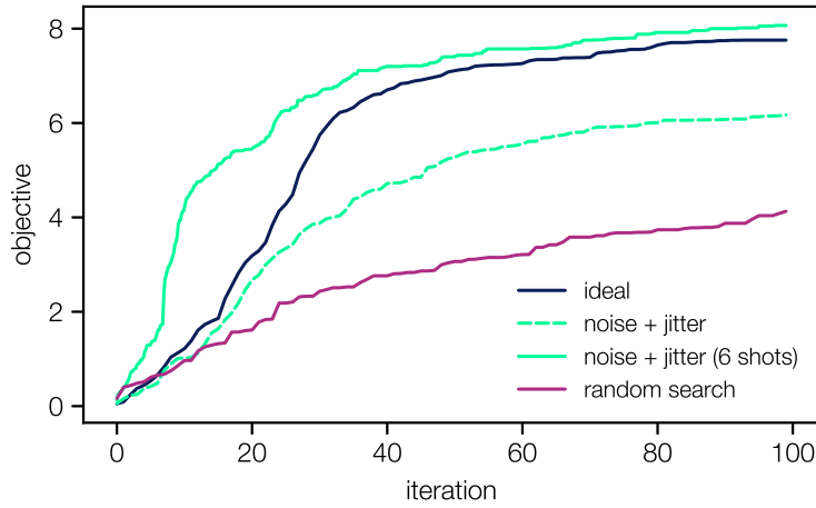
Figure 5.1 – Convergence tests for Bayesian optimization on LPA surrogate model (see section 3.2.4). Each line denotes the average performance (maximum objective found so far) over 50 independent optimization runs under each scenario. Experimental conditions (green lines) are simulated by introducing a fluctuation of 5 % on the laser energy and 150 \mu\text{m} on the focus position and by adding normally distributed noise ( \sigma = 0.1 ) to the measured objective. The different lines indicate different optimization approaches and scenarios: Standard Bayesian optimization of the ideal (blue) and noisy (green dashed) setup, purely random selection of different setpoints (red), and Bayesian optimization of the noisy setup but collecting six measurements at each setpoint (green).
