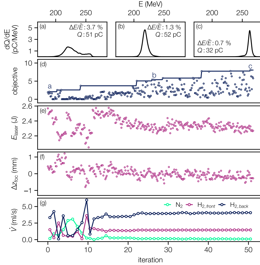
Figure 5.2 – Experimental optimization of LPA electron beams: (a-c) Measured energy spectra; (d) Measured objective function (dots) with the cumulative best result (blue line); (e-g) Input parameters with shot-to-shot measurements of the laser energy, focus position and gas flows for each input setting. The figure is adapted from [1].
