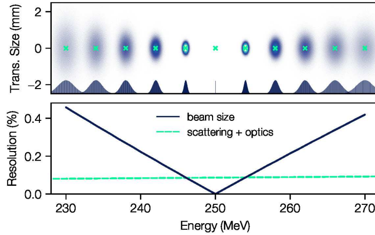
Figure 4.8 – Estimation of the electron spectrometer resolution for 250 MeV focused energy. (Top) Beam tracking simulations of monoenergetic beams at different energies (green crosses) with 4\text{ }\mu\text{m} source size and 1 mrad divergence. Blue curves indicate the projection onto the energy axis, the in-focus beam (250 MeV) is too small to be resolved in the plot. (Bottom) Energy resolution around the focused energy given by the rms beam size along the energy axis (blue, solid) and by the optical system and scattering effects in the vacuum chamber (green, dashed).
