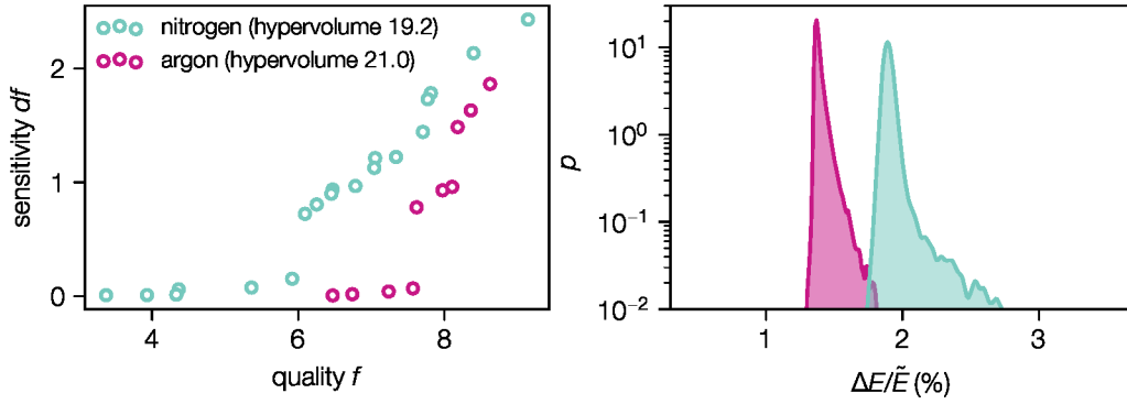
Figure 3.18 – Multi-objective optimization of the setup with nitrogen (green) and with argon (violet) as the dopant gas. Left: Obtained Pareto fronts of the quality objective f and the sensitivity objective df . Right: Energy spread stability of the most stable setpoints for each scenario under the influence of realistic laser jitter. The probability distributions are generated by sampling the surrogate models of the respective optimization runs. Both setpoints have comparable median energy with 550 MeV (nitrogen) and 556 MeV (argon).
