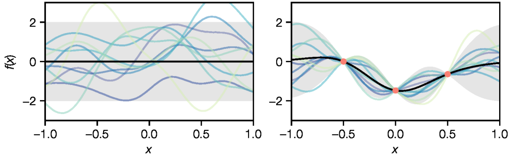
Figure 2.5 – Samples (colored lines) from a Gaussian process prior (left panel) and posterior (right panel) after conditioning on data (red dots). The black line indicates the mean of the Gaussian process and the gray area its 2\sigma confidence region. By conditioning the process its mean and confidence collapse so that the samples are forced through the data points which in this example are assumed to be free of noise.
