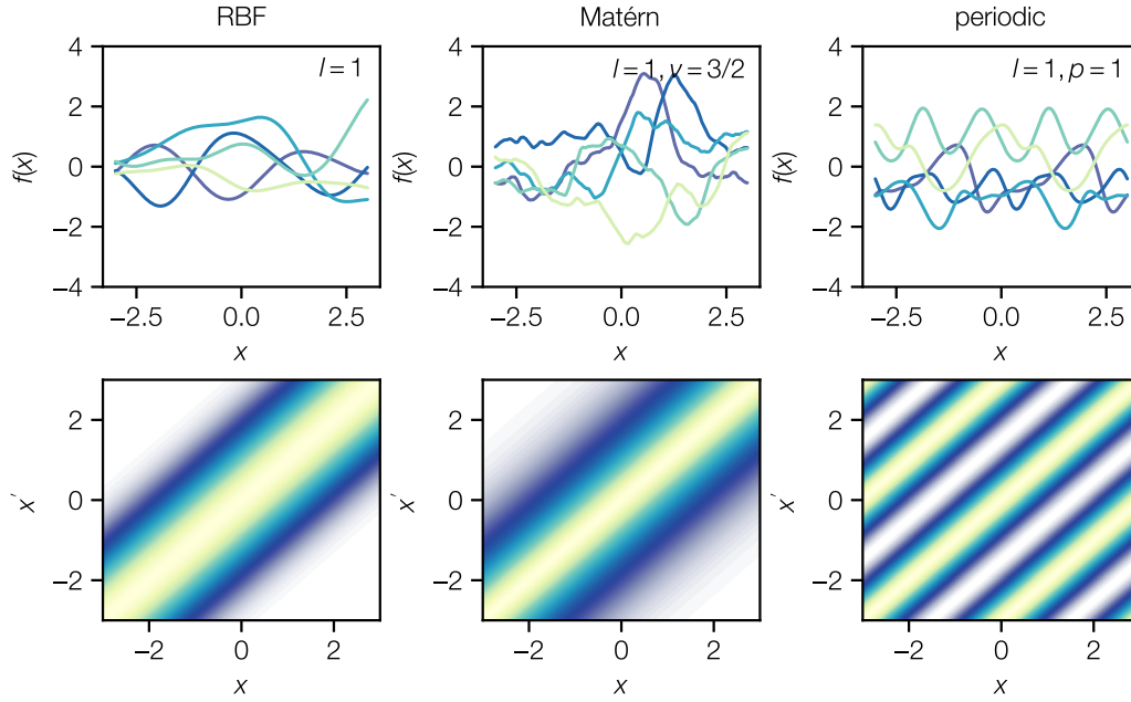
Figure 2.4 – Characteristics of different kernel functions. Samples from Gaussian processes with given kernels (top) and their corresponding covariance matrices (bottom).
