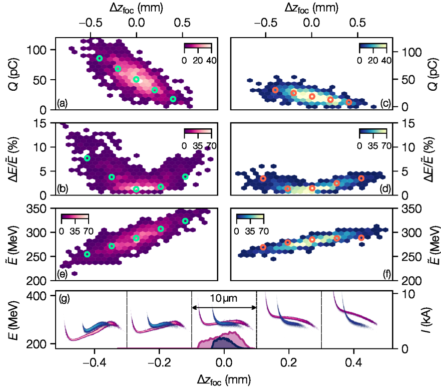
Figure 5.7 – Stability-optimized LPA: (a)-(f) Measured (heatmaps) and simulated (circles) correlations between the laser focus position and beam parameters for a typical reference (purple) and the stability optimized (blue) setting. Colormaps indicate the number of recorded events. (g) Longitudinal phase spaces from PIC simulations with the corresponding current profiles. The figure is adapted from [1].
