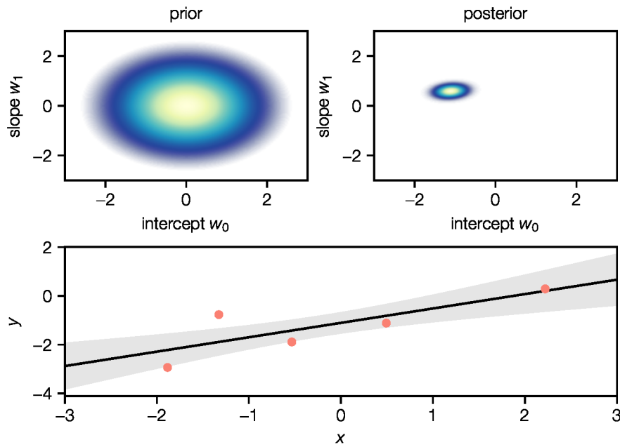
Figure 2.2 – Bayesian linear regression with noisy data samples (red dots). The prior distribution (upper left) expresses the belief that the model parameters w_0 and w_1 are close to zero. Conditioning the model on the data yields the posterior distribution (upper right) according to which the data most likely follows a model with finite slope and intercept. Bottom: Mean and confidence ( \pm two standard deviations) of the posterior predictive distribution (eq. (2.15)).
