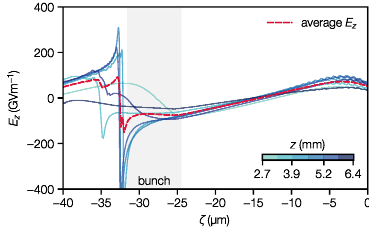
Figure 3.3 – Evolution of the accelerating field during the propagation through the plasma. Variations of the beam loading effect due to changes of the wakefield strength result in on average flattening of the field (red dashed line) over the majority of the bunch length (grey area). The colors of the lines indicates the corresponding position in the plasma source, see colorbar.
