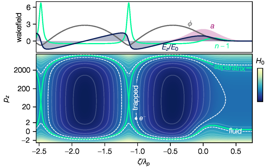
Figure 1.3 – Motion of electrons in a laser wakefield. Top: Wakefield properties according to eq. (1.18) for a driver with a_0 = 3 . Bottom: Phase space trajectories (\zeta, p_z) for different total energy H_0 . Figure adapted from [69].
