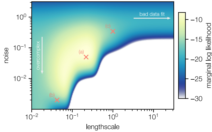
Figure 2.8 – Log marginal likelihood for data and example models from fig. 2.7 (crosses). Complex models with small lengthscales tend to overfit on the data. On the other end with too simple models with large lengthscales much information in the data is interpreted as noise. The marginal likelihood balances the data fit and model complexity.
