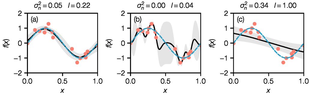
Figure 2.7 – Gaussian process models (RBF kernel) with different hyperparameters conditioned on the same data (red dots). Depending on the choice of lengthscale l and noise \sigma_n^2 of the covariance function the model is able to generalize the underlying sine function (blue) better or worse. Without noise (middle) the model requires a small lengthscale to account for all data points. This leads to erratic behavior of the mean when interpolating between the measured data. If the lengthscale is too large (right), the information in the data is interpreted as noise leading to a too simple model.
