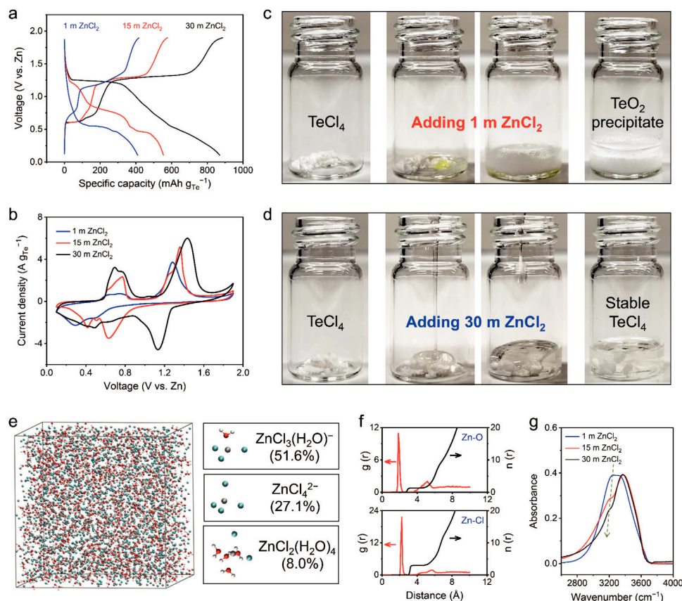
Figure 3. Te conversion chemistries in different electrolytes. a) GCD curves at 400 mA g Te −1 and b) CV curves at 1 mV s −1 of TeG in the ZnCl 2 electrolytes with different concentrations. c,d) Optical photos of adding 1 m ZnCl 2 (c) and 30 m ZnCl 2 into commercial TeCl 4 (d). e) Snapshot of the 30 m ZnCl 2 electrolyte and the typical local coordination structures of Zn in the molecular dynamics simulation. White atoms, red atoms, cyan atoms, and gray atoms are H, O, Cl, and Zn atoms, respectively. f) Radial distribution functions g ( r ) and integral profiles n ( r ) of Zn–O (of H 2 O) and Zn–Cl coordination in 30 m ZnCl 2 . g) FTIR spectra of the ZnCl 2 electrolytes with different concentrations.
