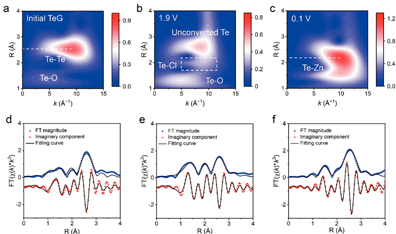
Figure 5. The EXAFS analysis of TeG at different states. Wavelet-transformed Te K-edge EXAFS of a) initial TeG, b) fully charged TeG (1.9 V), and c) fully discharged TeG (0.1 V). EXAFS data (points) and fit curve (line) in R-space (Fourier transform [FT] magnitude and imaginary component) for d) initial TeG, e) fully charged TeG (1.9 V), and f) fully discharged TeG (0.1 V). The data are k^3 -weighted without phase correction.
