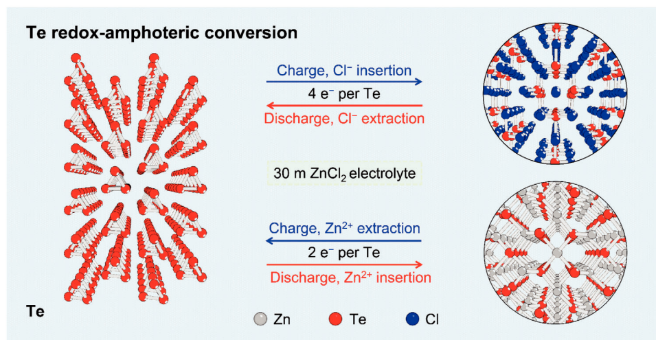
Figure 1. Schematic showing the Te redox-amphoteric conversion process. During the redox-amphoteric conversion, Te can be either oxidized to \text{TeCl}_4 or reduced to \text{ZnTe} .
