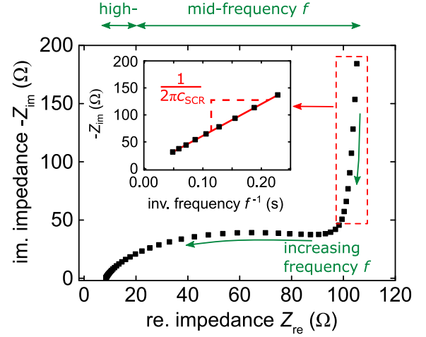
Fig. 1. Characteristic Nyquist plot of a porous silicon electrode in 1 \text{mol l}^{-1} perchloric acid at a static applied potential of 0.2 V with frequencies in the range of 100 kHz to 4.3849 Hz. The high- (100 to 1 kHz) and the mid-frequency range (1000 to 4 Hz) are indicated. In the inset the data points of the vertical increase regime at the lowest frequencies (red indication) are plotted versus their inverse frequency f^{-1} . A linear fit to the data points yields a capacitance of c_{\text{SCR}} = 0.21 \text{mF} .
