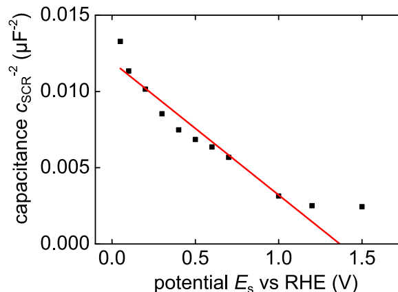
Fig. 3. Mott-Schottky plot of a bulk silicon electrode in 1 mol l -1 perchloric acid. The capacitance determined by EIS is plotted as c_{\text{SCR}}^{-2} versus the respective static potential E_s . c_{\text{SCR}} is determined via EIS measurements with frequencies in the range of 1 MHz to 500 MHz and static potentials in the range of 0.05–1.5 V. A linear fit to the Mott-Schottky plot yields a flatband potential of E_{\text{fb}} = 1.4 \pm 0.1 V and a carrier concentration of N_a = (2.6 \pm 0.3) \cdot 10^{19} \text{ cm}^{-3} . The linear fit is only performed up until a potential of 1.0 V. The line of the fit is then prolonged to mark the flatband potential at c_{\text{SCR}}^{-2} = 0 .
