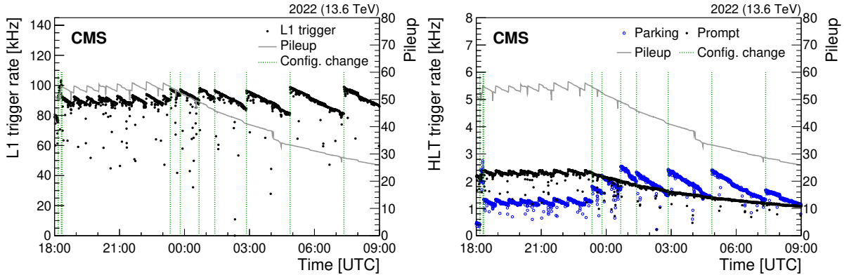
Figure 54: Total L1 (left) and HLT (right) trigger rates, and the number of pileup interactions, shown as a function of time for a representative LHC fill during 2022. The rates for the promptly reconstructed core physics (black solid markers) and B parking (blue open markers) data streams are shown separately in the right panel. Occasional lower rates are observed due to transient effects, such as the throttling of the trigger system in response to subdetector dead time [9]. Changes in the trigger configuration are indicated by vertical green dashed lines.
