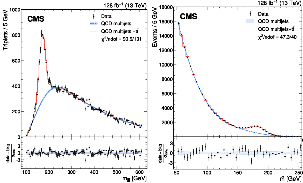
Figure 6: The distribution of m_{3j} for the resolved three-jet search (left), and average jet mass ( \tilde{m} = (m_1 + m_2)/2 ) for the merged three-parton search (right), adapted from Ref. [67]. Both analyses use PF jets. The peak around 170 GeV in both distributions corresponds to the all-hadronic decay of the top quark. The data (points) are compared to the background-only prediction (blue) and the full background fit including simulations of the top quark resonance (red).
