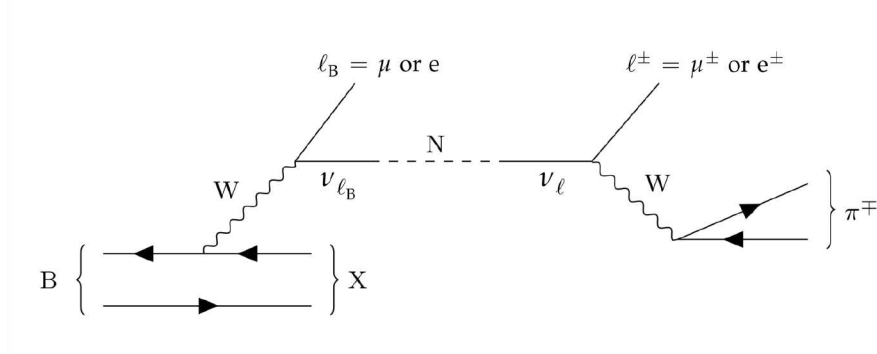
Figure 48: Feynman diagram of a semileptonic decay of a B meson into the primary lepton ( \ell_p ), a hadronic system (X), and a SM neutrino, which then mixes with a heavy neutrino (N). The N decays weakly into a charged lepton \ell^\pm and a charged pion \pi^\mp , forming a vertex displaced from the pp interaction point. Taken from Ref. [158].
