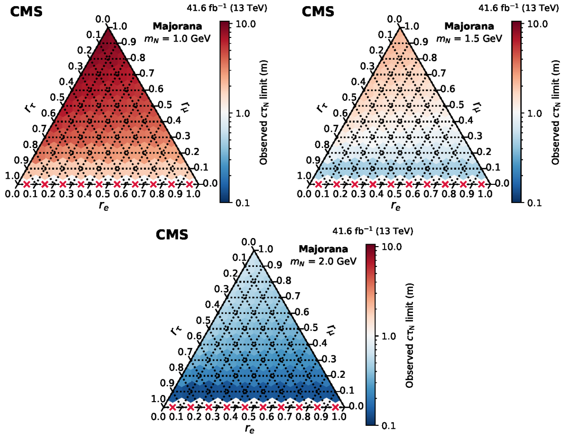
Figure 50: Observed limits on \tau_N as a function of the coupling ratios (r_e, r_\mu, r_\tau) for fixed N masses of 1 GeV (upper left), 1.5 GeV (upper right), and 2 GeV (lower center), in the Majorana scenario. A red cross indicates that no exclusion limit was set for that point. The tick orientation indicates the direction of reading. Taken from Ref. [158].
