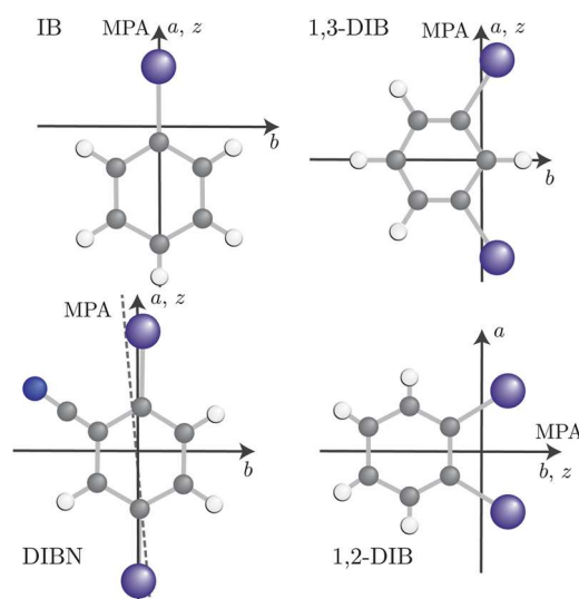
FIG. 1. Sketches of the molecules IB, DIBN, 1,3-DIB, and 1,2-DIB. For IB and 1,3-DIBN the most polarizable axis (MPA) is parallel to the a axis, for DIBN it forms an angle of 5^\circ with the a axis, and for 1,2-DIB the MPA is parallel to the b axis. The molecule-fixed z axis is indicated in the respective sketches.
