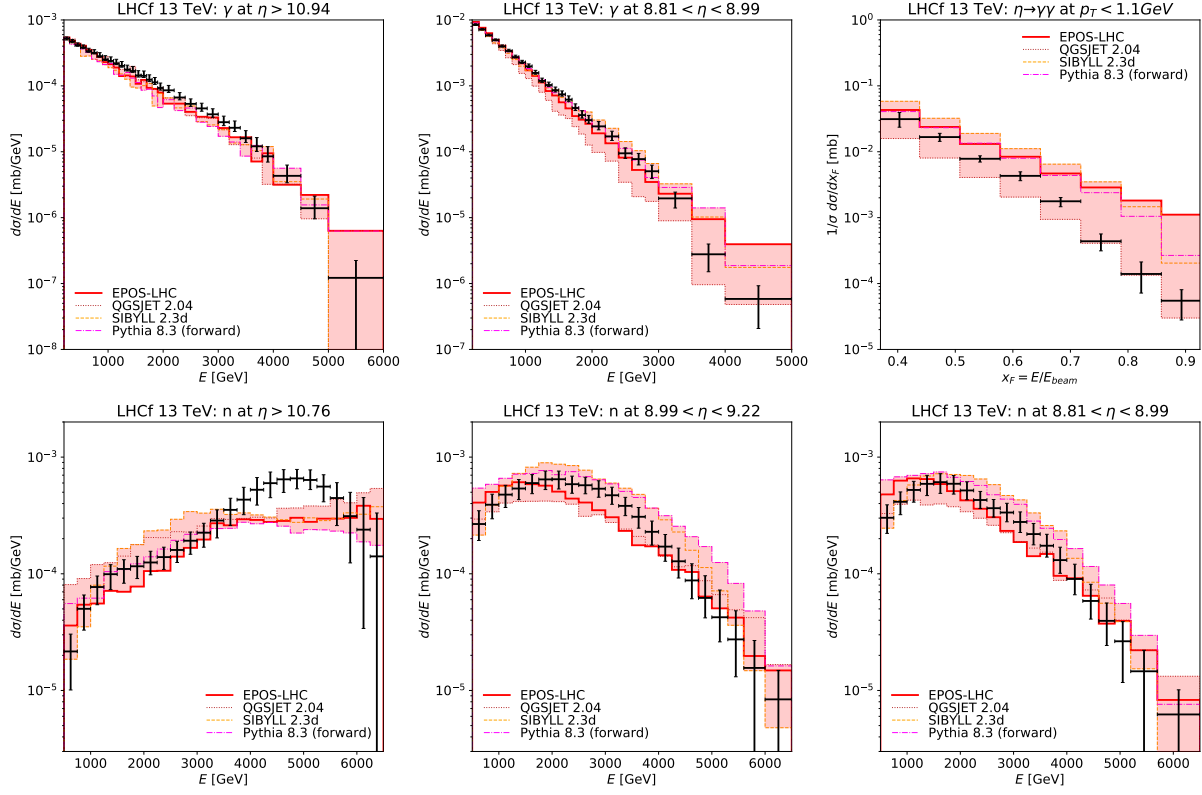
FIG. 2. Forward Particle Energy Spectra at LHCf and Model Predictions. The energy spectra of forward photons [34] (upper left and upper center), \eta -mesons [35] (upper right), and neutrons [36] (lower left, lower center, and lower right) measured by LHCf in different pseudorapidity bins, compared to the predictions of the event generators EPOS-LHC [29], SIBYLL [30], QGSJET [31], and PYTHIAforward [32]. The shaded bands correspond to the spread of the event generator predictions.
