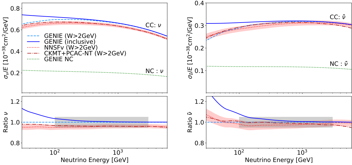
FIG. 4. Top: Muon neutrino (left) and anti-neutrino (right) CC interaction cross sections as functions of the incoming neutrino energy, as obtained using GENIE [37], NNSFv [51], and CKMT+PCAC-NT [52], as indicated. For comparison, we show the neutral-current (NC) cross section prediction of GENIE in dotted green. The electron neutrino cross section prediction is approximately the same, differing by less than 0.1% for E_\nu > 100 \text{ GeV} , and the tau neutrino cross section is \lesssim 20\% smaller, due to the tau mass. The red-shaded bands show the NNSFv uncertainty band. Bottom: Muon neutrino (left) and anti-neutrino (right) CC cross sections normalized to the GENIE W > 2 \text{ GeV} results. The gray bands correspond to flat 6% uncertainties in the energy range 100 \text{ GeV} < E_\nu < 3 \text{ TeV} .
