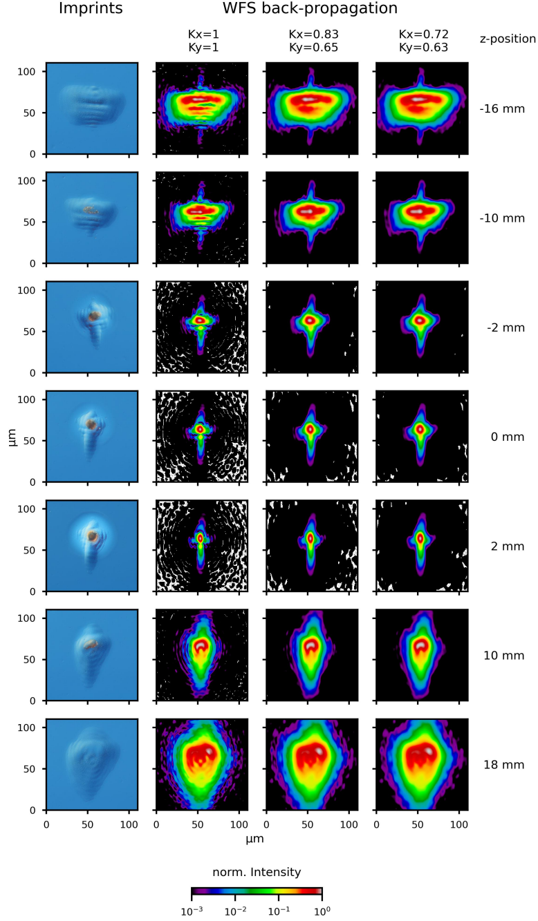
Fig. S3. Comparison of chosen PMMA imprints and intensity profiles back-propagated with various degrees of coherence from WFS measured beam profiles. First column: Nomarski microscope images of PMMA imprints in sample no. 9 measured along the caustic. Last three columns: Back-propagated intensity profiles along the caustic retrieved from a measurement with 100 pulses averaged on the WFS CCD chip. Different degrees of coherence K_x in horizontal and K_y in vertical direction were used ( K_x=0.83^a , K_y=0.65^a and K_x=0.72^a , K_y=0.63^a ). Intensities are shown in logarithmic color scale to show the good agreement, also in boundary areas, of the beam profile shape and structure with the PMMA imprints. Propagation direction of the FEL light is from top to bottom. Focus position corresponds to z = 0 mm, wavelength is 13.48 nm with 12 undulators in use whereby the last 6 were quadratic tapered ( z_u = 30 m).
