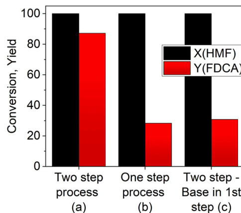
Fig. 6. Comparison of one- and two-step process for the oxidation of crude HMF solution (0.3 M HMF, 50 bar air, HMF:M 230:1). (a): 1st step: 100 °C, 1.5 h, 1 eq. \text{Na}_2\text{CO}_3 ; 2nd step: 140 °C, 4 h, 3.3 eq. NaOH. (b): 140 °C, 5.5 h, 3.3 eq. NaOH, 1 eq. \text{Na}_2\text{CO}_3 . (c): 1st step: 100 °C, 1.5 h, 3.3 eq. NaOH, 1 eq. \text{Na}_2\text{CO}_3 ; 2nd step: 140 °C, 4 h.
