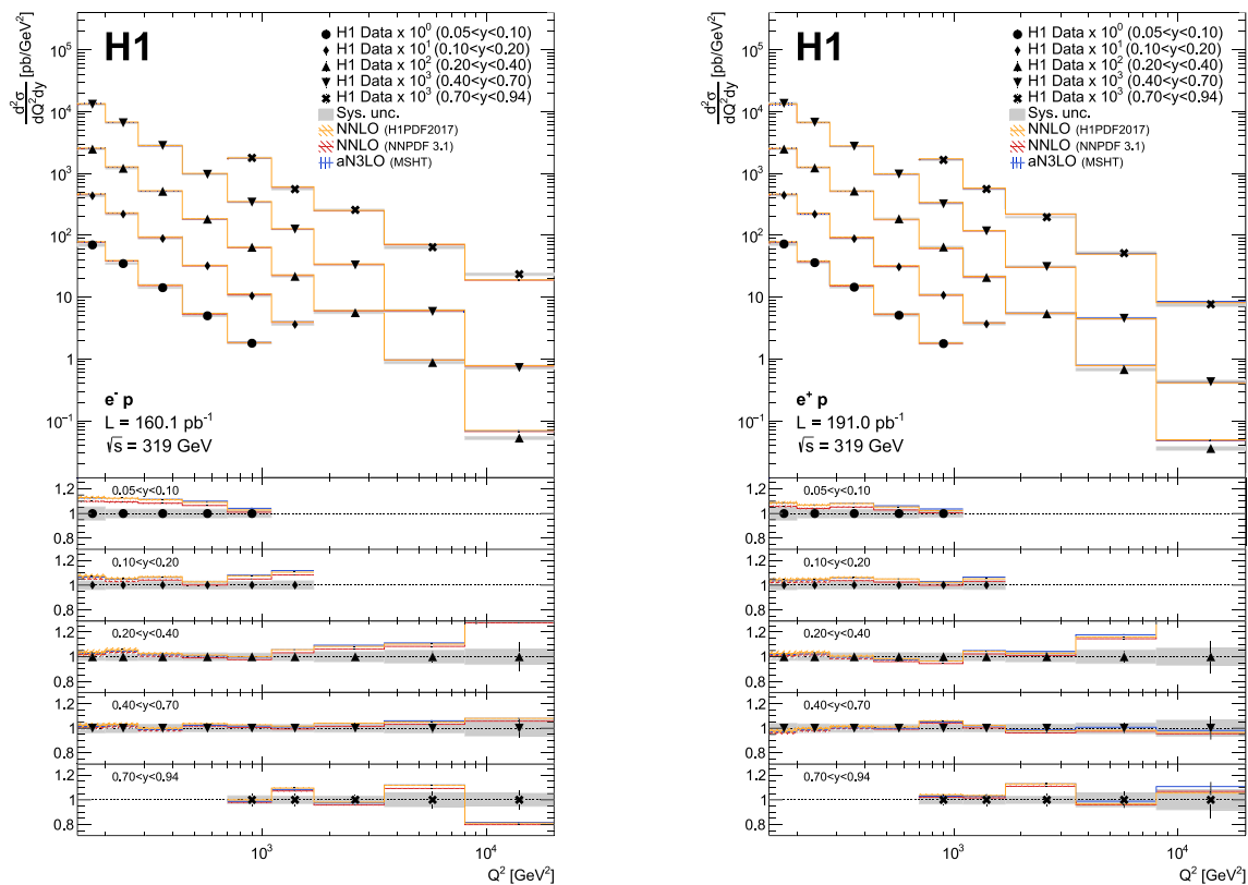
Fig. 13 The double-differential inclusive neutral current DIS cross section \frac{d^2 \sigma_{\text{NC}}}{dQ^2 dy} for e^-p (left) and e^+p (right) scattering in the kinematic region 150 \leq Q^2 < 20000 \text{ GeV}^2 and 0.05 \leq y < 0.94 . The data are displayed as full circles, the vertical error bars indicate statistical uncertainties, while systematic uncertainties are displayed as shaded area. Different y ranges are indicated by different markers, and are displaced vertically by a constant factor as indicated in the legend.
