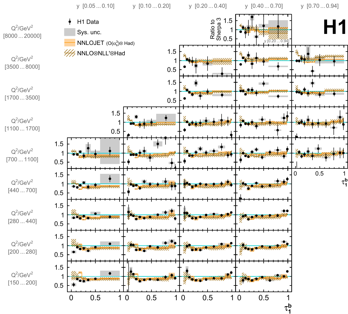
Fig. 8 The ratio of data and NNLOJET ( \mathcal{O}(\alpha_s^3) ) and NNLO+NLL'@Had predictions to the Sherpa 3.0 predictions for the triple-differential cross section \frac{d^3\sigma}{d\tau_1^b dQ^2 dy} . See Fig. 7 caption for further details. The data are displayed as full circles, the vertical error bars indicate statistical uncertainties, while systematic uncer-
