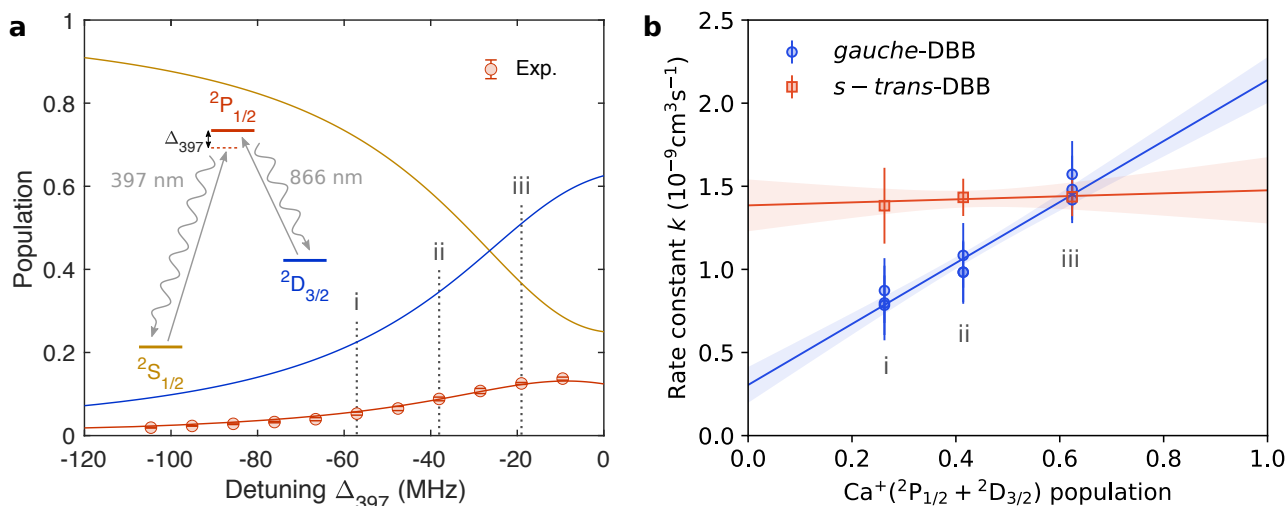
Fig. 4: Ca^+ state-dependent rate coefficients. a , Dependence of the ^2S_{1/2} , ^2P_{1/2} and ^2D_{3/2} state populations of Ca^+ on the detuning of the 397 nm cooling laser. Solid lines correspond to the theoretical model and data points represent experimental ^2P_{1/2} state population determined from the ion fluorescence at 397 nm. The vertical lines labelled i–iii, denote the detunings at which rate measurements were performed. Inset: energy-level diagram of Ca^+ . b , Results of the state- and conformer-resolved rate measurements at the detunings i–iii of a . The lines are linear least-squares fits interpolating between bimolecular rate coefficients for Ca^+ in the ground (S) and excited states (P+D). Shaded areas correspond to a 90% confidence region. Error bars are fit errors of the individual rate measurements.
