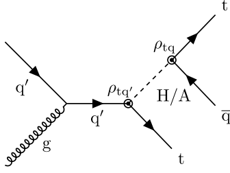
Fig. 1. Representative Feynman diagram for t\bar{t}q ( q = u, c ) production through a new scalar (H) or pseudoscalar (A) Higgs boson. In this analysis, events with q = q' are considered.
