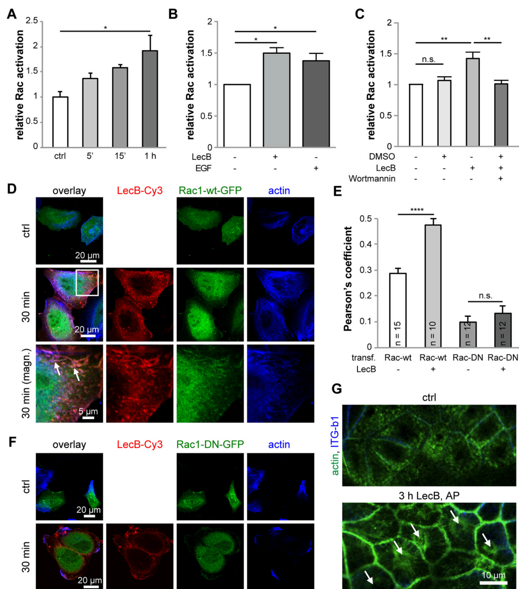
FIG 3 Apical LecB stimulation leads to Rac activation and actin rearrangement. (A) The activation of Rac upon apical LecB treatment of MDCK cells was measured using a Rac123-G-LISA assay; n = 3 . (B) H1975 cells were treated with LecB or EGF (20 nM), and Rac activation was measured using a Rac123-G-LISA assay; n = 3 . (C) H1975 cells were treated with LecB and wortmannin (100 nM), and Rac activation was measured using a Rac123-G-LISA assay; n = 6 . (D to F) H1975 cells transfected with Rac1-wt-GFP (green) (D) or Rac1-DN-GFP (green) (F) were treated with LecB-Cy3 (red) as indicated, fixed, and stained for actin with phalloidin-Atto 647 (blue). (D) White arrows point to ruffle-like structures where LecB, Rac1-wt-GFP, and actin colocalized. (E) The Pearson's colocalization coefficient between Rac1-wt-GFP or Rac1-DN-GFP and actin in cells untreated or treated with LecB-Cy3 was determined in individual cells, and the average was calculated. (G) MDCK cells treated with LecB as indicated were fixed and stained with phalloidin-Atto 488 to stain actin (green) and \beta 1-integrin (blue). Lateral confocal cross sections along the apical poles of the cells are displayed.
