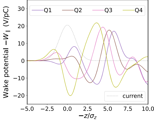
FIG. 7. CSR wakefield per quarter at the third bend (B3) of ch1 for a Gaussian bunch with \sigma_z = 96 \mu\text{m} . The symbol Qi indicates the i th quarter of the bend. The wake potentials are calculated using impedance data from the CSRZ code.
