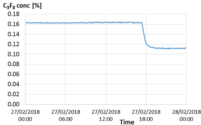
Fig. 10. Change in C_3F_8 concentration in the Pixel detector envelope following a reduction of operating temperature from -5^\circ\text{C} to -20^\circ\text{C} on February 27, 2018.
