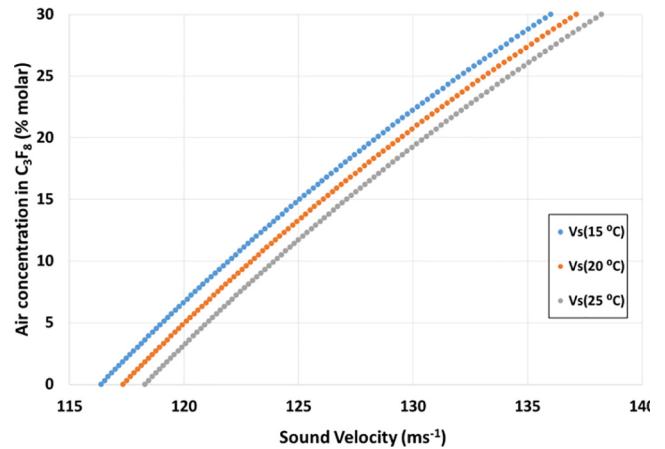
Fig. 7. Sound velocity dependence on air concentration in C_3F_8 vapor at three temperatures of the degassing sonar and a pressure of 300 \text{ mbar}_{\text{abs}} .
