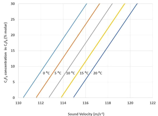
Fig. 12. Variation of sound velocity with molar % C_2F_6 concentration in C_3F_8 over the range 0–30% at several temperatures of the superheated zeotropic blend: pressure 0.1 MPa.
