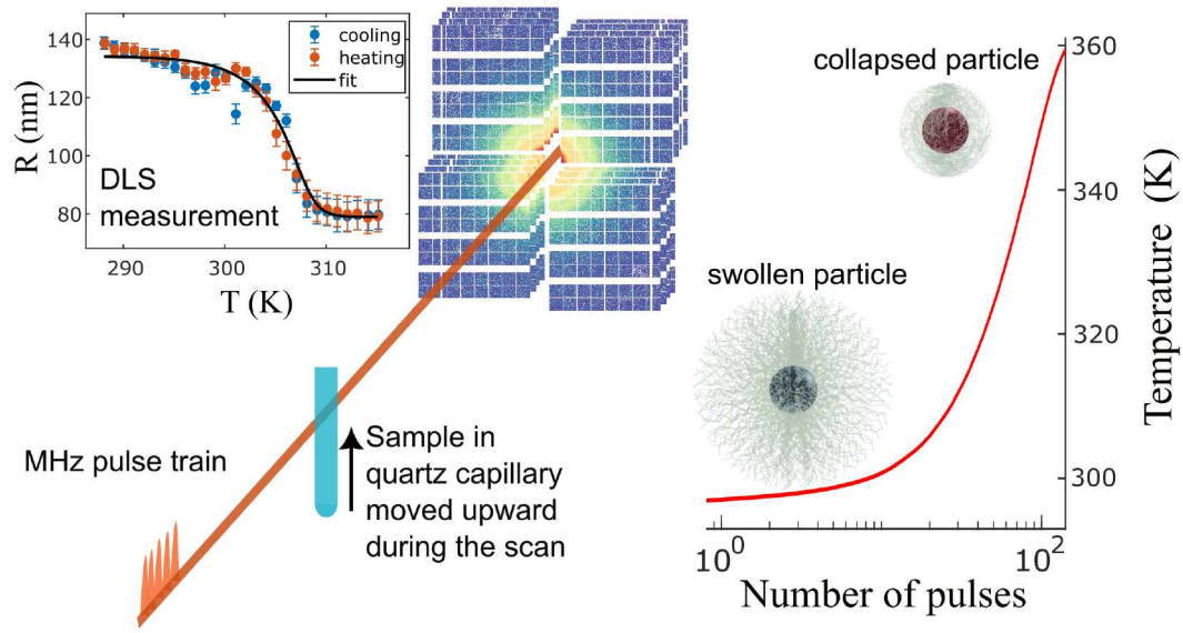
Figure 1: Conceptual scheme of the experiment. Central panel: the train of X-ray pulses reaches the sample and heats it up in a controlled manner (red line in the right plot). If the silica nanoparticles are covered by PNIPAm, then the series of pulses will trigger the transition from the swollen hydrophilic to the collapsed hydrophobic state. In the top-left plot a typical DLS characterization of one of our core-shell system is displayed, specifically a sample at high cross-linker concentration and thin shell thickness of 34 nm in the collapsed state.
