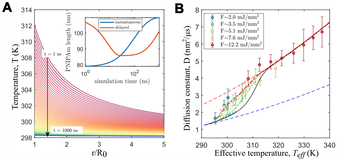
Figure 5: Results from time-resolved model. (a): Calculated temperature as a function of r/R_0 and t after a temperature jump of 14 K. In the inset the calculated elongations of the PNIPAm chains are reported for a situation in which there is no delay in the response (blue) and a delay of 10 ns and 800 ns in the collapse and reswelling, respectively. (b): Model results for 1.1 MHz data and thick shell 8 wt% BIS compared with the experimental data (model:dot-dashed lines; data: circles). The dashed lines are limit values that mark the diffusion of swollen (blue) and collapsed (red) particles. The black line represents the instantaneous response limit.
