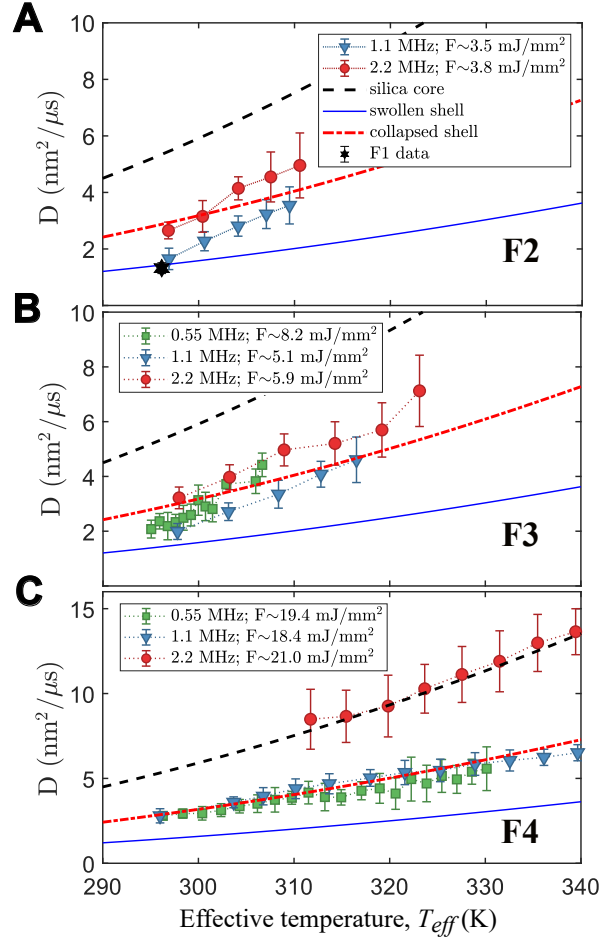
Figure 4: Diffusion constant for samples with thick shell and BIS 8 wt% as a function of T_{\text{eff}} for different repetition rates and different fluences. (a) Low fluence limit of regime F2, for comparison the measured diffusion constant obtained from an F1 run is also reported (black star). Due to the limited signal to noise ratio only data for 1.1 MHz and 2.2 MHz are reported. (b) Intermediate fluences (regime F3). (c) High fluences (regime F4). The lines represent the limit values for the completely swollen (solid blue), fully collapsed (dash-dotted red) and pure silica core (dashed black) state.
