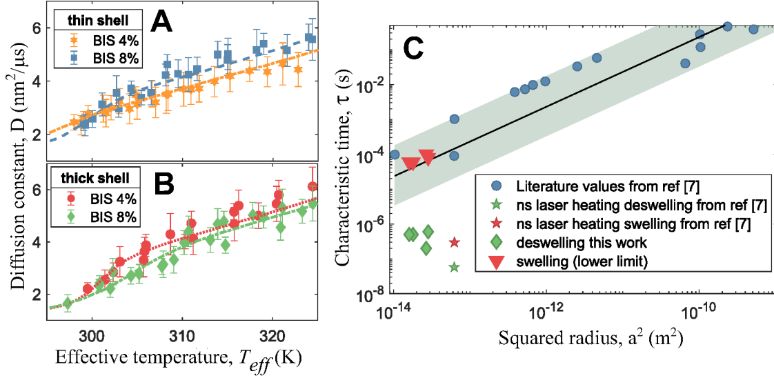
Figure 6: Fitted models and results compared with literature. (a): data for thinner shell and different BIS concentrations, data at 8 wt% BIS (blue squares) are obtained from 1.125 MHz runs while 4 wt% BIS (orange hexagons) were obtained from 0.55 MHz runs because for technical reasons it was not possible to measure F3 data for the latter sample. (b): data for 1.125 MHz runs for thicker shell at different BIS concentrations of 4 wt% (red circles) and 8 wt% (green diamonds). The fits shown here used a fixed \tau_{swell} = 80 \mu s (dashed lines of respective colours). (c): Results of the present work, diamonds and triangles, reported together with literature values from (7) (stars) and references therein (circles). The line is a linear fit to the literature data and the shaded area is the confidence band.
