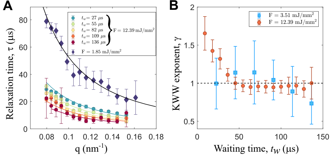
Figure 3: Relaxation times and KWW exponents for samples with thin shell and BIS 8 wt%. (a) Relaxation times as a function of q for two fluences. For F = 1.85 \text{ mJ/mm}^2 the average over the whole TTCM is displayed. The black line is the fit of the Stokes-Einstein relation and returns a diffusion constant of 1.9 \pm 0.1 \text{ nm}^2/\mu\text{s} . The colored data are the pulse-resolved average relaxation times for F = 12.2 \text{ mJ/mm}^2 . (b) KWW exponent at different t_w for two fluences of F = 12.2 \text{ mJ/mm}^2 and F = 3.51 \text{ mJ/mm}^2 .
