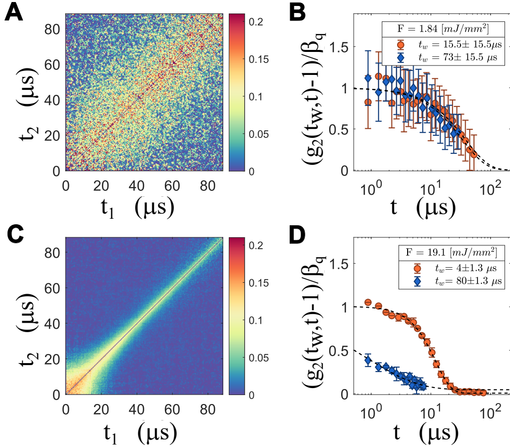
Figure 2: Examples of the observed dynamics at q=0.087 \text{ nm}^{-1} in two fluence regimes. (a) and (c) show the TTCM for a low fluence ( 1.84 \text{ mJ/mm}^2 ) and a high fluence ( 19.12 \text{ mJ/mm}^2 ) measurement. (b) and (d) show the corresponding time-resolved correlation functions g_2(t_w, t) at two t_w : orange circles shows a t_w at the beginning of the train, blue diamonds a t_w at the end of the train. To fit the blue points in (d) both baseline and contrast were kept fixed at the values obtained from the fit at the beginning of the train.
