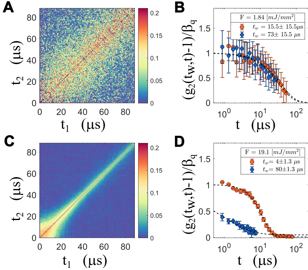
Figure 2: Examples of the observed dynamics at q=0.087 \text{ nm}^{-1} in two fluence regimes. (a) and (c) show the TTCM for a low fluence ( 1.84 \text{ mJ}/\text{mm}^2 ) and a high fluence ( 19.12 \text{ mJ}/\text{mm}^2 ) measurement. (b) and (d) show the corresponding time-resolved correlation functions g_2(t_w, t) at two t_w : orange circles shows a t_w at the beginning of the train, blue diamonds a t_w at the end of the train. To fit the blue points in (d) both baseline and contrast were kept fixed at the values obtained from the fit at the beginning of the train.
