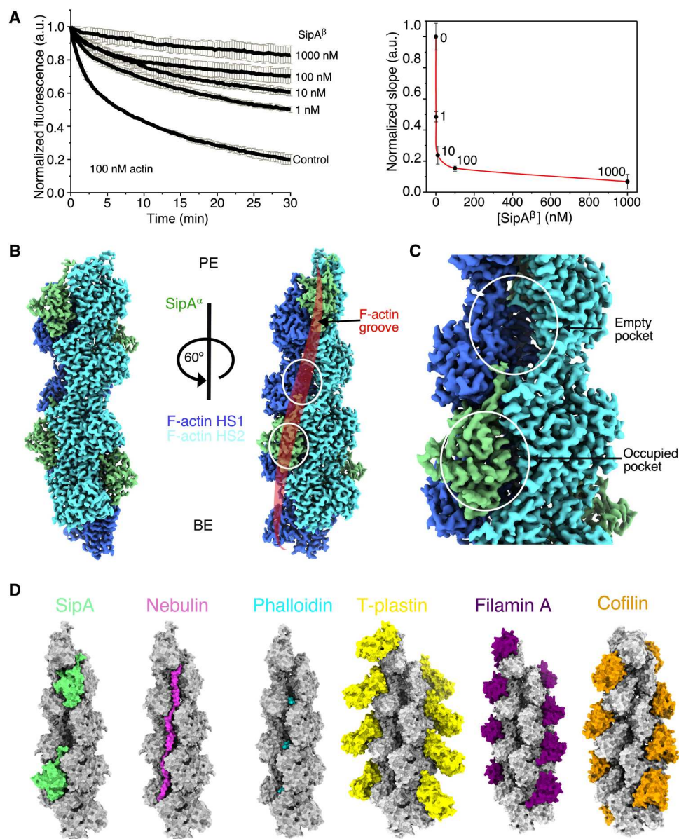
Fig. 2. SipA stabilizes F-actin under substoichiometric conditions and binds in a unique pattern. (A) Time course of F-actin depolymerization induced by dilution in the presence of SipA \beta (left). SipA \beta -free buffer was used as negative control (left). Normalized and averaged initial slopes of dilution-induced depolymerization assays were plotted against the concentration of SipA \beta (right). Data points and error bars indicate means \pm SD from three independent experiments. a.u., arbitrary units. (B) Cryo-EM structure of SipA \alpha bound to F-actin. Two F-actin helical strands decorated by SipA \alpha are colored dark blue and light blue, and SipA \alpha molecules are shown in light green. The pointed end (PE), barbed end (BE), F-actin groove, and F-actin pocket are indicated. HS, helical strand. (C) Zoomed-in view of SipA \alpha well-anchored inside the F-actin pocket. The adjacent empty pocket and the occupied pocket are indicated. (D) Surface representations of F-actin (gray) with different interaction partner: nebulin–F-actin [Protein Data Bank (PDB): 7QIM] (25), phalloidin–F-actin (PDB: 7BTI) (24), filamin A–F-actin (PDB: 6D8C) (27), T-plastin–F-actin (PDB: 7R94) (26), and cofilin–F-actin (PDB: 6VAO) (28).
