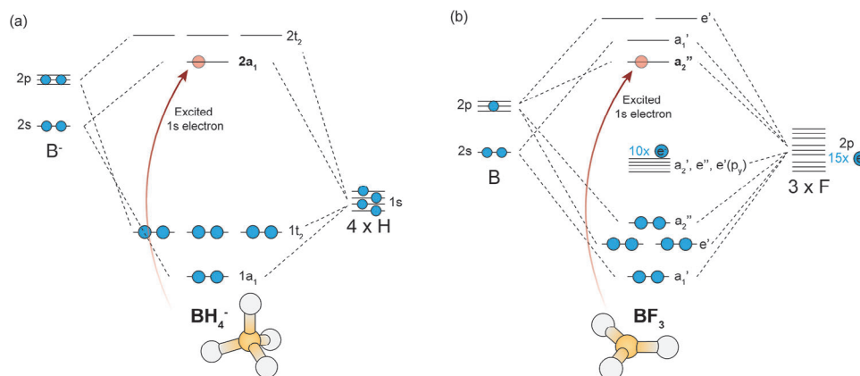
Figure 4. Schematic representation of the molecular orbital diagrams of a) \text{BH}_4^- and b) \text{BF}_3 based on symmetry-adapted linear combinations (SALCs). The corresponding molecular geometries, that is, tetrahedral for \text{BH}_4^- and trigonal planar for \text{BF}_3 , are provided as well.
