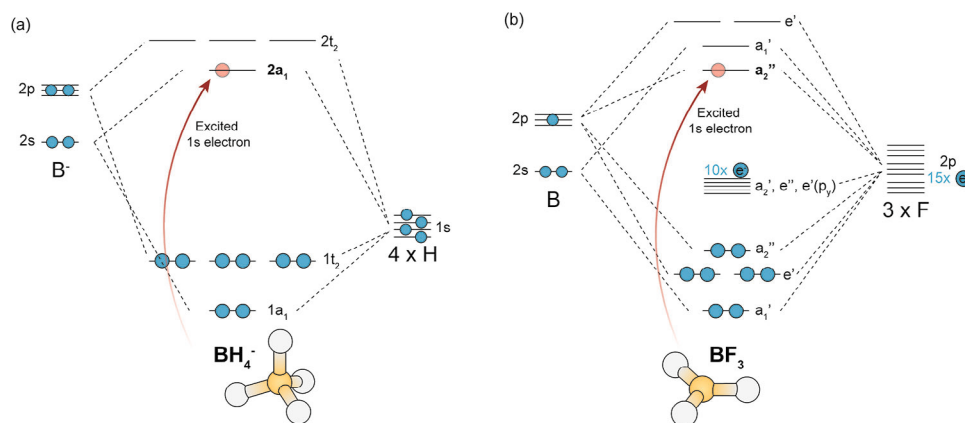
Figure 4. Schematic representation of the molecular orbital diagrams of a) \text{BH}_4^- and b) \text{BF}_3 based on symmetry-adapted linear combinations (SALCs). The corresponding molecular geometries, that is, tetrahedral for \text{BH}_4^- and trigonal planar for \text{BF}_3 , are provided as well.
