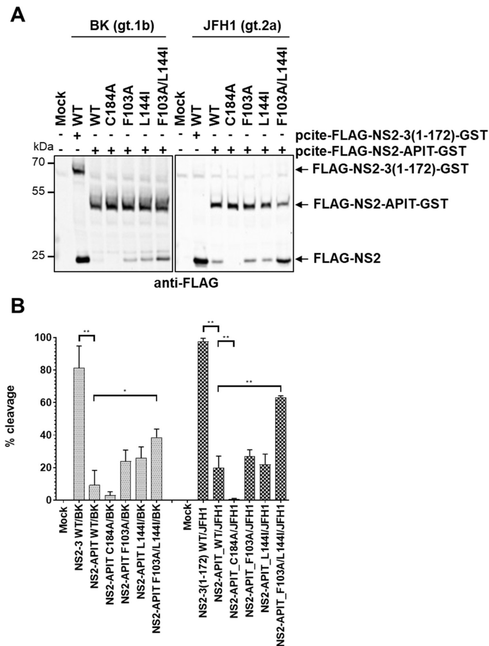
Fig 5. The amino acid exchanges F103A and L144I lead to a stimulation of the intrinsic NS2 pro cleavage efficiency in the absence of the NS3 cofactor in two different HCV genotypes. (A) Analysis of the intrinsic NS2 pro activity in the MVA/T7 pol expression system in Huh7-T7 cells. NS2-mediated cleavage of FLAG-NS2-NS3(1–172)-GST or FLAG-NS2-APIT-GST polypeptide fragments was analyzed by Western blotting using FLAG-specific antibodies. One representative blot from three independent experiments is shown. Molecular mass standards are shown on the left. Positions of the uncleaved precursors FLAG-NS2-NS3(1–172)-GST or FLAG-NS2-APIT-GST and cleavage product FLAG-NS2 are indicated by arrows on the right. (B) Quantification of NS2-protease mediated cleavage efficiencies (percent of cleavage calculated as percent of cleavage product over the sum of uncleaved precursor plus cleaved product) from lysates subjected to immunoblotting using infrared fluorescent-labeled secondary antibodies and the Odyssey SA imaging system (LI-COR). Background was subtracted from FLAG-specific signals of uncleaved precursors and cleavage product using the corresponding signal of the mock sample. Mean and standard deviation of NS2 pro cleavage efficiencies from three independent experiments are presented. WT: wild-type; mock: transfection control without plasmid DNA. Asterisks indicate statistically significant differences in comparison to WT (* p < 0.05 ; ** p < 0.01 ).
