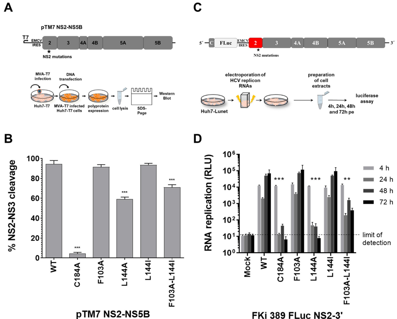
Fig 8. The NS2 F103A/L144I double mutation is reducing NS2-NS3 cleavage efficiencies in the NS2-NS5B context and is reducing robust RNA replication of a NS2-5B JFH1 replicon. (A, upper panel) Scheme of pTM7-NS2-NS5B/JFH1. (A, lower panel) schematic of the NS2-NS3 cleavage assay. 6 \mu g of the indicated pTM7-NS2-NS5B/JFH1 plasmids were transfected into MVA/T7 pol -infected Huh7-T7 cells. Lysates were analyzed by SDS/PAGE-Western blotting using HCV anti-NS2 and anti-NS3 antibodies, respectively. (B) Quantification of the NS2-NS3 cleavage. Western blot signals of NS2, NS3 and uncleaved NS2-NS3 of three independent Western blots were quantified by ImageJ software and the percentage of NS2-NS3 cleavage (% NS2-NS3 cleavage) was calculated. Mean and standard deviations of NS2-NS3 cleavage efficiencies are presented. (C, upper panel) Experimental setup for RNA replication assay. Huh7 Lunet cells were electroporated with 10 \mu g of respective FKi-389_FLuc-NS2-3'/JFH1 RNAs. Lower panel, determination of viral replication. HCV RNA replication kinetics were quantified at 4, 24, 48 and 72 h post electroporation by measuring firefly luciferase activity (relative light units, RLU). Graphs are representative results of three independent experiments with standard deviations. WT: wild-type; mock: electroporation control without RNA. Asterisks indicate statistically significant differences in comparison to WT (* p < 0.05 ; ** p < 0.01 ; *** p < 0.001 ).
