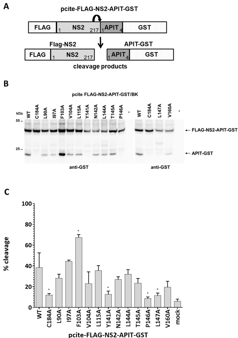
Fig 2. Re-analyzing of NS2 Pro surface residues in the NS2-APIT-GST context revealed F103A as a stimulating determinant for the intrinsic NS2 Pro activity in the absence of the NS3 cofactor. (A) Schematic representation of the pcite-FLAG-NS2-APIT-GST expression construct used to analyze the NS2 Pro activity in the absence of its cofactor NS3. Cleavage of FLAG-NS2-APIT-GST results in generation of FLAG-NS2 and APIT-GST. (B) Indicated pcite-FLAG-NS2-APIT-GST plasmids were transfected into Huh7-T7 cells and expressed by the MVA/T7 pol expression system. One representative blot from three independent experiments is shown. Molecular mass standards are shown on the left. Positions of the FLAG-NS2-APIT-GST and the cleavage product APIT-GST are indicated on the right. WT: wild-type; mock: transfection control without DNA. (C) NS2 protease cleavage efficiencies. Signals of uncleaved FLAG-NS2-APIT-GST and the cleavage product APIT-GST were quantified by ImageJ software from three Western blots to calculate the percentage of FLAG-NS2-APIT-GST cleavage. Mean and standard deviations of NS2 cleavage efficiencies from three independent experiments are presented. Asterisk indicate statistically significant differences in comparison to WT (* p < 0.05 ).
