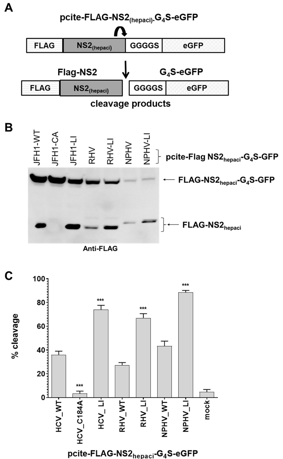
Fig 7. Leucine-to-isoleucine exchanges in other hepaciviral NS2 proteins corresponding to mutation HCV NS2 L144I are activating the intrinsic NS2 pro activity. (A) Scheme of pcite-FLAG-NS2 hepaci -G 4 S-eGFP reporter construct to analyze the intrinsic NS2 protease activity of related mammalian hepaciviruses. (B) Indicated pcite plasmid
