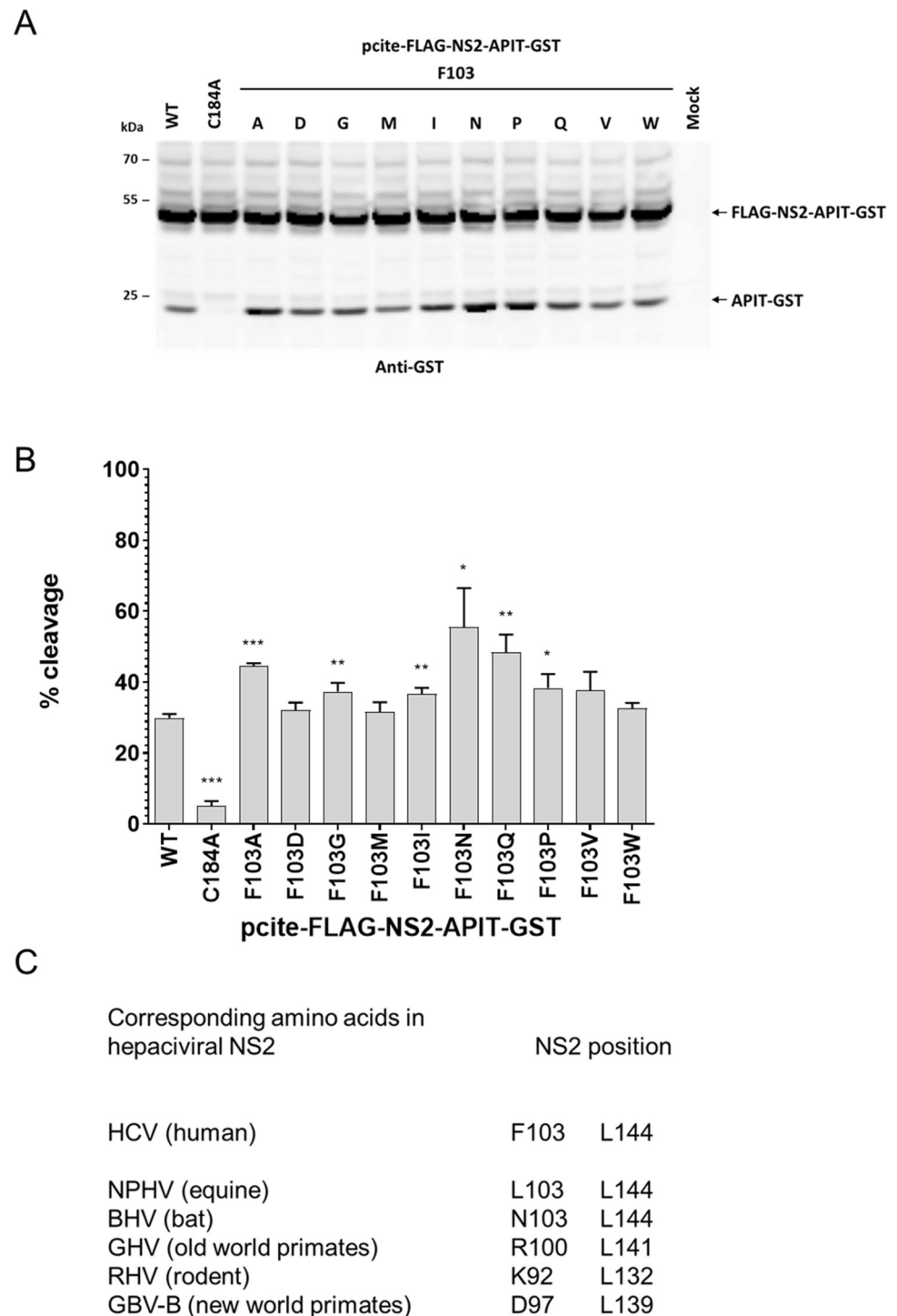
Fig 4. F103 permutation analysis revealed a broad spectrum of amino acids is allowing intrinsic NS2 protease cleavage. (A) Analysis of the intrinsic NS2 pro activity in the MVA/T7 pol expression system in Huh7-T7 cells. NS2-mediated cleavage of FLAG-NS2-APIT-GST was analyzed by Western blotting using GST-specific antibodies. (B) NS2 pro cleavage efficiencies. Signals of uncleaved FLAG-NS2-APIT-GST and the cleavage product APIT-GST were quantified by ImageJ from three Western blots to calculate the percentage of NS2-APIT-GST cleavage. Mean and standard deviations of NS2 pro cleavage efficiencies from three independent experiments are presented. Molecular mass standards are shown on the left. Positions of the uncleaved precursors FLAG-NS2-APIT-GST and the cleavage product APIT-GST are indicated on the right. WT: wild-type; mock: transfection control without plasmid DNA. (C) Conservation of HCV F103- and L144-corresponding NS2 residues in indicated mammalian hepatitis virus species
