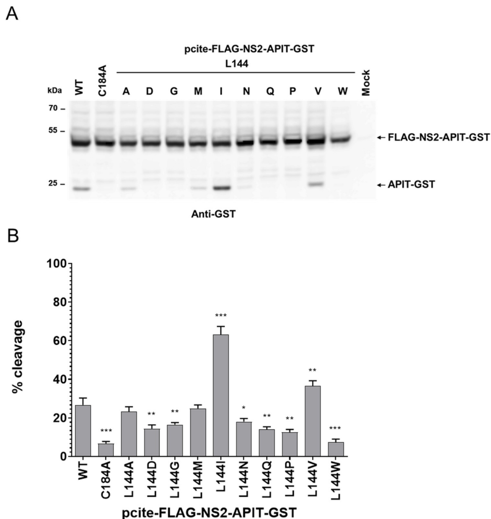
Fig 3. The amino acid exchange L144I is stimulating the intrinsic NS2 pro cleavage efficiency in the absence of the NS3 cofactor. (A) Analysis of the intrinsic NS2 pro activity assay in the MVA/T7 pol expression system in Huh7-T7 cells. NS2-mediated cleavage of FLAG-NS2-APIT-GST/BK was analyzed by Western blotting using GST-specific antibodies. One representative blot from three independent experiments is shown. (B) NS2 pro cleavage efficiencies. Signals of uncleaved FLAG-NS2-APIT-GST and the cleavage product APIT-GST were quantified by ImageJ software from three Western blots to calculate the percentage of NS2-APIT-GST cleavage. Mean and standard deviations of NS2 pro cleavage efficiencies from three independent experiments are presented. Molecular mass standards are shown on the left. Positions of the uncleaved precursor FLAG-NS2-APIT-GST and the cleavage product APIT-GST are indicated on the right. WT: wild-type; mock: transfection control without plasmid DNA. Asterisks indicate statistically significant differences in comparison to WT (* p < 0.05 ; ** p < 0.01 ; *** p < 0.001 ).
