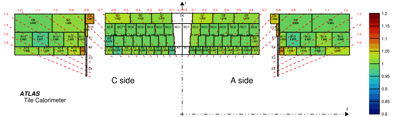
Figure 24: Visualisation of the TileCal in the (z, r) plane showing the 2017 estimated values of the ratios R_r of the cells of a given ring r (see the text). The values are obtained by maximising the likelihood function in Eq. (12). The statistical uncertainty in each determination is about 0.5%.
