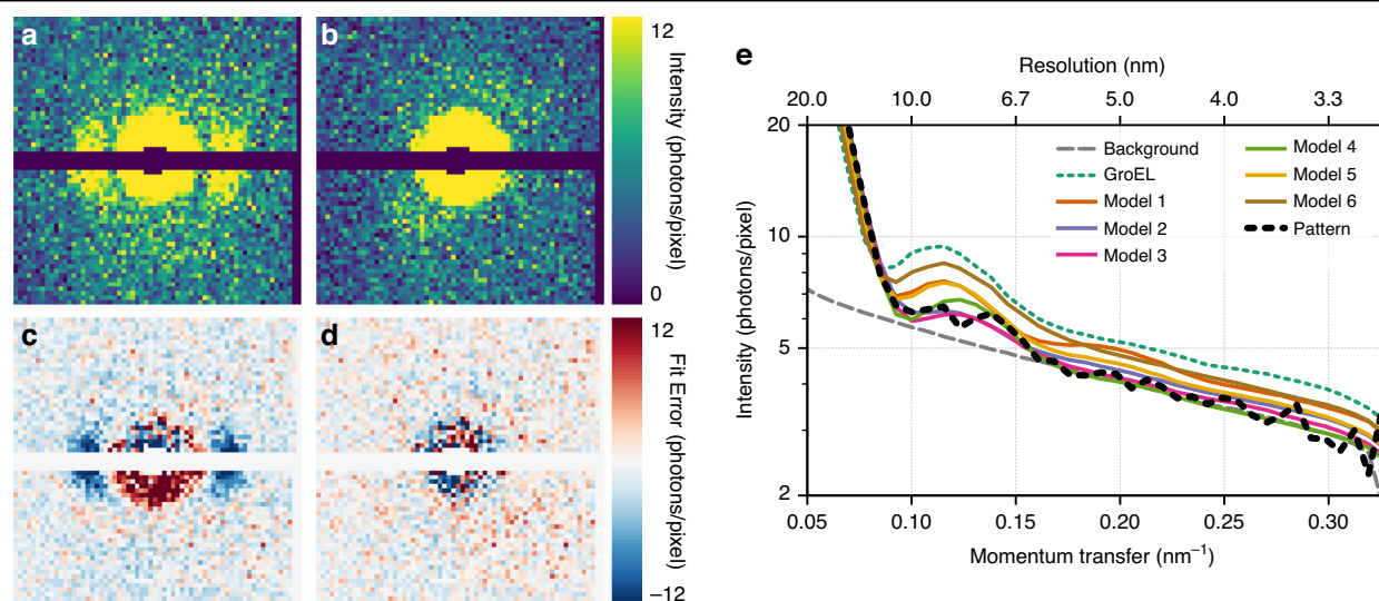
Fig. 5 Pattern comparisons. a Simulated diffraction from the dry GroEL particle in the orientation that best matches the measured pattern. Patterns are plotted after Poisson sampling to make the patterns comparable with the single pattern shown in Fig. 2c. b A significantly better fit is achieved from density model 3. c, d Fit error between the measured pattern compared to c the simulated diffraction from the dry GroEL particle and d model 3. e Radial average of the background to illustrate the difference between the models, the best-fitting diffraction from the crystal structure of GroEL (dotted green line), each density model (solid coloured lines) and the measured pattern (dotted black line). The dry molecule predicts too much intensity outside of the central speckle, whereas water models 2, 3 and 4 follow the data much closer. The images ( a–d ) and the pixels of ( e ) correspond to 64 \times 64 downsampled patterns
