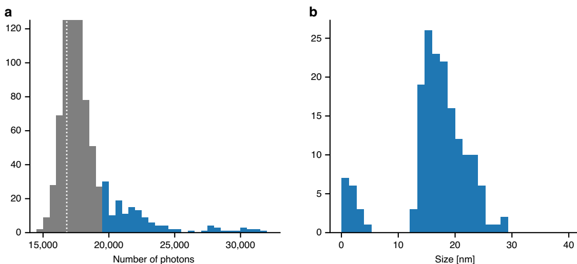
Fig. 3 Data classification. a Histogram showing the number of photons per pattern. The dotted line marks the average strength of the background. The strong peak around 17,000 contains mainly pure-background shots, but most diffraction patterns above 19,000, marked in blue, have diffraction signal from a sample. b Histogram of the size of the sample in all patterns with more than 19,000 photons. The peak at 15 nm matches the size of GroEL and the second smaller peak below 5 nm consists of particularly strong pure-background shots
