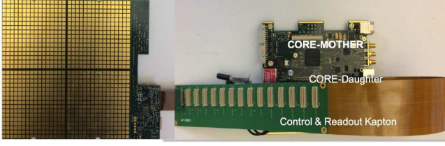
Figure 1. Picture of the complete DAQ attached to a single layer.
