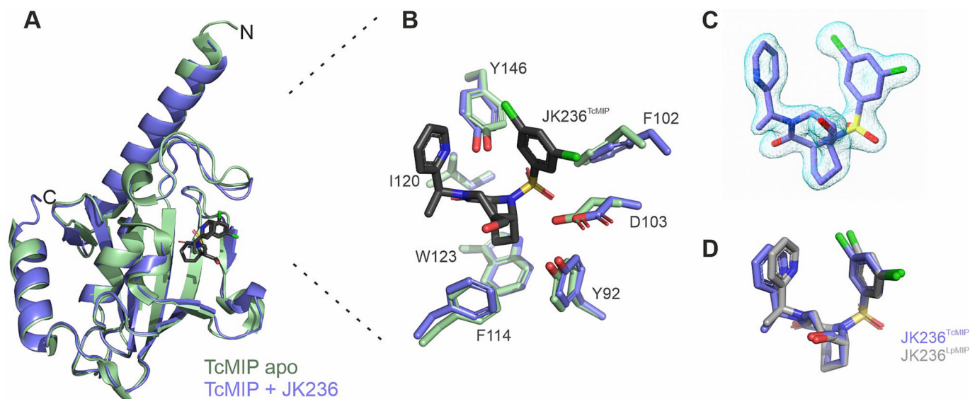
Fig. 8. Trypanosoma cruzi MIP in complex with a [4.3.1]-aza-bicyclic sulfonamide inhibitor. (A) Overlay of the crystal structures of apo TcMIP (green, PDB: 1JVW) and JK236-bound TcMIP (blue, PDB: 8BK4). (B) Active site residues in the apo or JK236-bound TcMIP. The ligand is shown in black. (C) Electron density for JK236 bound to TcMIP. The 2Fo-Fc electron density maps are shown in light blue mesh at 3 \sigma . (D) Comparison of the inhibitor binding stance in TcMIP (blue) and LpMIP 77–213 (grey). For details, see also Fig. S9. (For interpretation of the references to color in this figure legend, the reader is referred to the web version of this article.)
