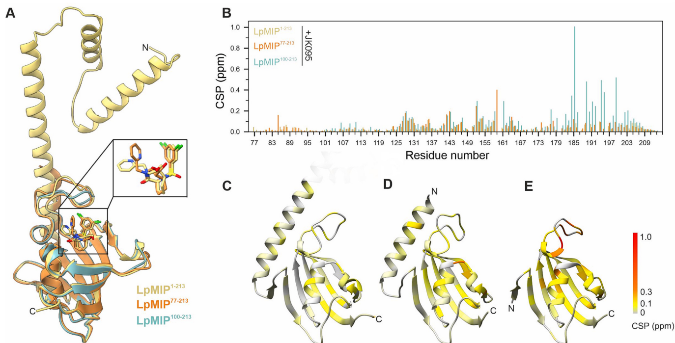
Fig. 5. Stalk helix affects interaction of LpMIP FKBP-like domain with a [4.3.1]-aza-bicyclic sulfonamide inhibitor. (A) Overlay of the X-ray crystal structures of LpMIP 1-213 (full-length), LpMIP 77-213 and LpMIP 100-213 co-crystallized with JK095 (PDB IDs: 8BJD, 8BK5, 8BK6). For the LpMIP 1-213 homodimer, only one subunit is shown. LpMIP 100-213 also crystallizes as a dimer, but no clear density for the ligand was obtained (for details see main text and compare Fig. S8). In the zoom-in, not that in LpMIP 77-213 , the hydroxymethyl group of JK095 was found to adopt two different conformations. (B) Chemical shift perturbations in the FKBP-like domain of 15 N-labeled full-length LpMIP (yellow), LpMIP 77-213 (orange) and LpMIP 100-213 (teal) upon titration with JK095. For better comparison between the three constructs, a unified scale normalized to the maximal shift value in the FKBP-like domain across all three data sets was used. (C–E) JK095-induced chemical shift perturbations within the FKBP-like domain plotted on crystal structures of full-length LpMIP (C), LpMIP 77-213 (D) and LpMIP 100-213 (E). (For interpretation of the references to color in this figure legend, the reader is referred to the web version of this article.)
