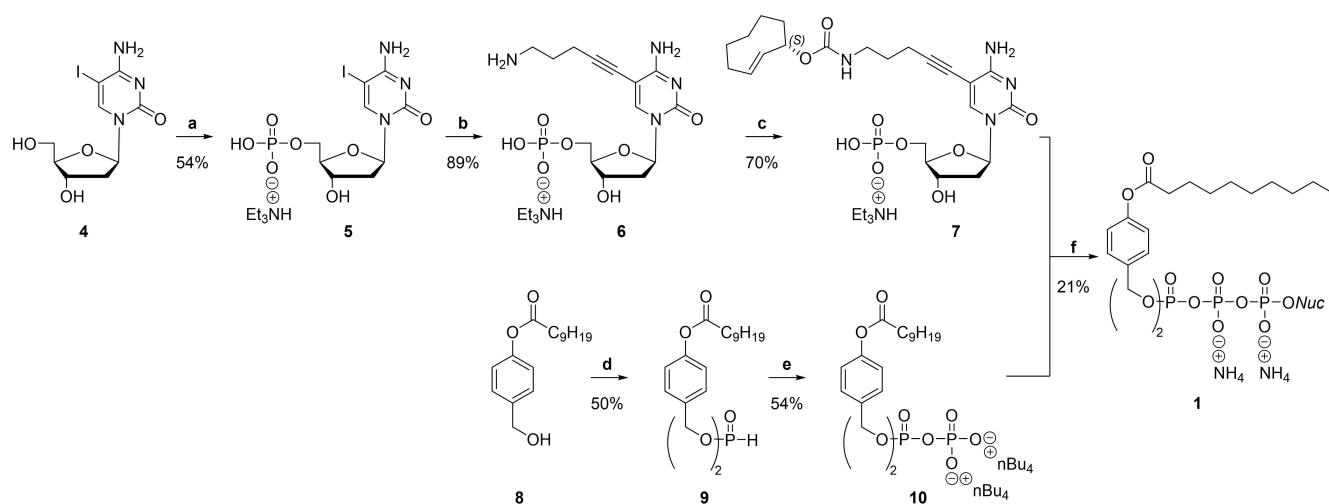
Scheme 1. Synthesis of the TriPPP compound \gamma -(bis-C9AB)-2TCOa-dCTP 1 . Reagents and conditions: a) i) \text{P}(\text{O})\text{Cl}_3 (4.4 equiv), pyridine (4.8 equiv), \text{H}_2\text{O} (2.8 equiv) in \text{CH}_3\text{CN} (18.9 equiv), 0^\circ\text{C} , 10 min; ii) 5-iodo-2'-deoxycytidine, 0^\circ\text{C} ; iii) ice water, \text{NH}_4\text{HCO}_3 (pH = 8); iv) \text{RP}_{18} column chromatography v) ion-exchange to TEA; b) \text{Pd}_2(\text{dba})_3 (5.4 mol%), tri(2-furyl) phosphine (12 mol%), \text{CuI} (15 mol%), 1-amino-4-pentyne, \text{Et}_3\text{N} (7 equiv), \text{DMSO} , 55^\circ\text{C} , 1 h; c) 2TCOa-NHS, \text{Et}_3\text{N} , \text{DMSO} , rt, 30 min; d) diphenyl phosphonate, pyridine, 40^\circ\text{C} ; e) i) NCS, \text{CH}_3\text{CN} , 50 – 60^\circ\text{C} ; ii) 0.4 M mono-tetra- n -butylammonium phosphate in \text{CH}_3\text{CN} , rt; f) i) TFAA, \text{Et}_3\text{N} , \text{CH}_3\text{CN} , 0^\circ\text{C} , 10 min; ii) 1-methylimidazole, \text{Et}_3\text{N} , \text{DMF} , 0^\circ\text{C} to rt; iii) NMP (TEA salt) in \text{DMF} , \text{CH}_3\text{CN} , rt, 3 h; iv) \text{RP}_{18} column chromatography, ion-exchange to ammonia, \text{RP}_{18} column chromatography.
