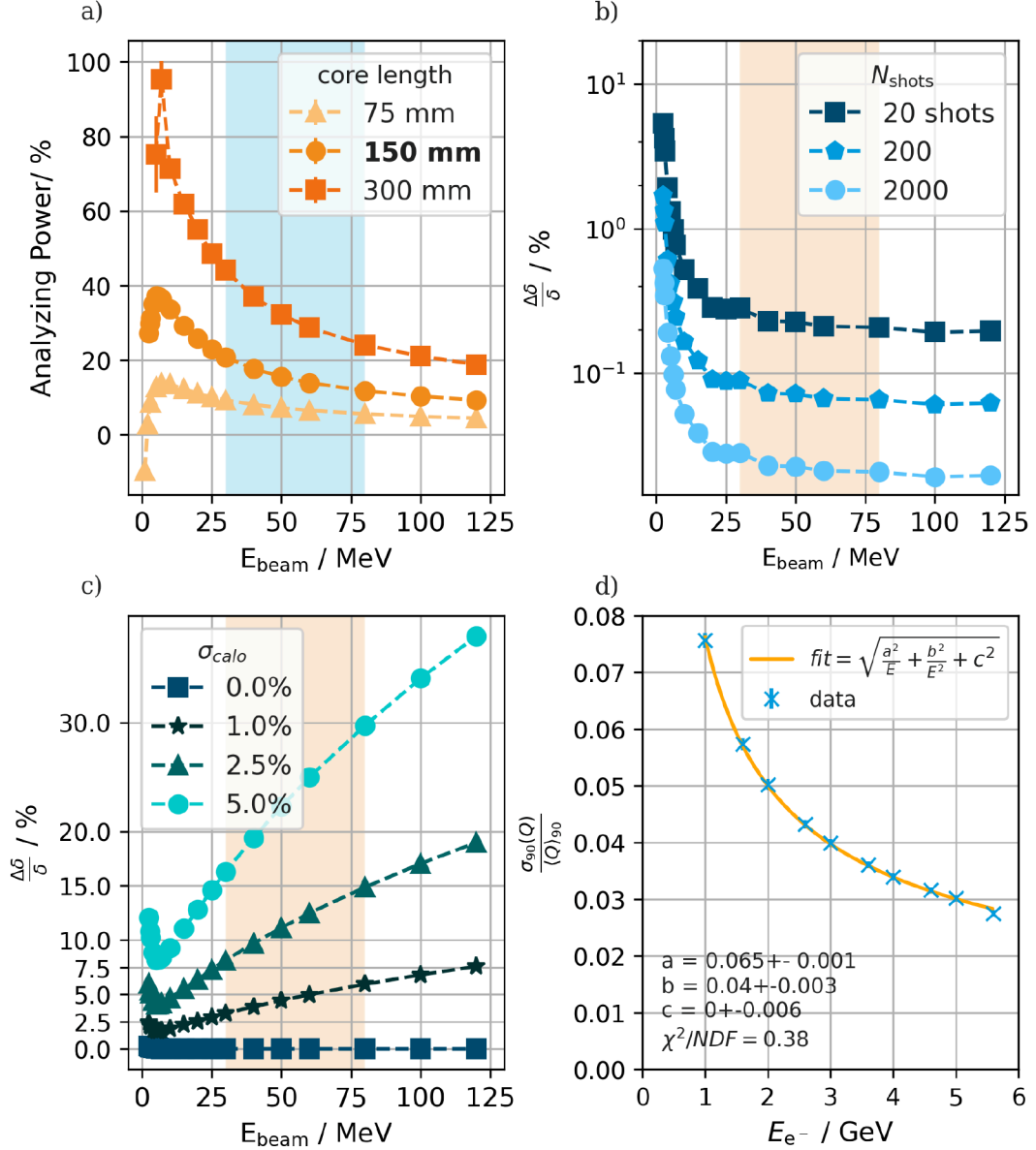
Figure 2: a) Analysing power over electron beam energy for different absorber thicknesses. P_{e^-} = 1 , P_{Fe} = \pm 1 . b) relative statistical precision of the expected asymmetry for different numbers of laser shots. N_{e^-}^{\text{sim}}/\text{bunch} = 5 \times 10^5 , core = 150 mm, d_{\text{conv}} = 1.75 mm, Q_{\text{expected}} = 3 pC, P_{e^-} = 1 , P_{Fe} = \pm 1 , \sigma_{\text{calo}} = 0 . c) relative statistical uncertainty of the expected asymmetry including different energy resolutions of the calorimeter. d) Energy resolution of the LEAP calorimeter. RMS-90 of the measured charge divided by the mean-90 over electron beam energy.
