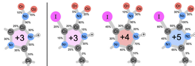
Fig. 7 Percentage of broken bonds between each atom except for hydrogen in triply-, quadruply- and quintuply-charged protonated \text{INimH} and triply-charged \text{NimH} molecules noted in the dynamics simulations.
