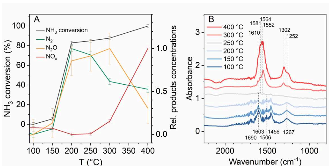
Figure 5. Results of operando DRIFTS measurements for PtA-IW-700: A – catalytic data, products determined by a mass spectrometer; B – DRIFTS spectra recorded at different temperatures.
