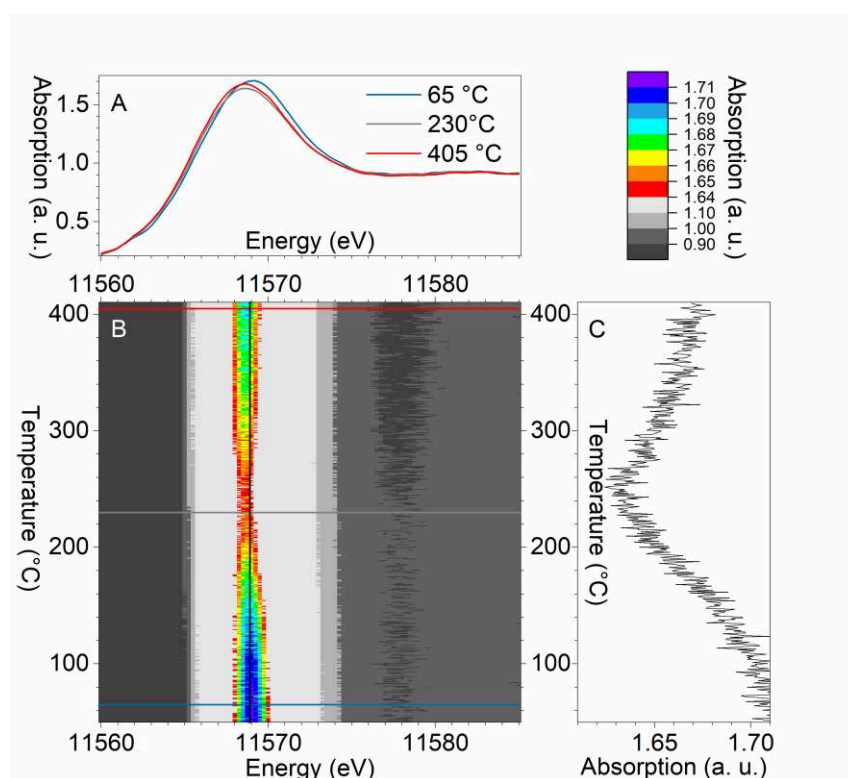
Figure 6. Contour plot for Pt L_3 normalized operando XANES spectra of PtA-IW-500 recorded during the second heating in the reaction mixture (500 ppm \text{NH}_3 and 10 % \text{O}_2 , inert balance). A – energy profiles of the contour plot at three different temperatures that corresponded to the spectra with the most different shapes (see a comparison with Pt and \text{PtO}_2 references in figure 4A). B – the contour plot. C – X-ray absorption profile at the energy near the maximum absorption intensity (11568.9 eV).
