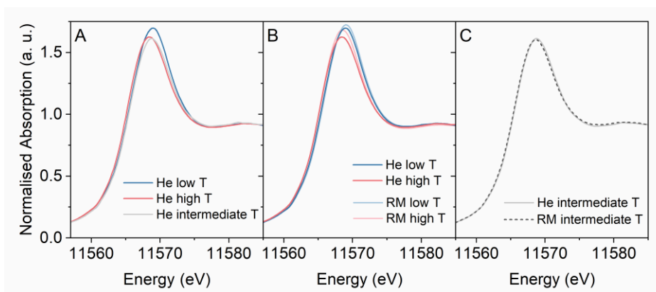
Figure 8. The MCR-derived most distinct spectral components for the Pt L_3 XANES spectra of PtA-IW-500: A – in He atmosphere; B – in He atmosphere compared to the ones dominating in the reaction mixture (RM) at high and low temperatures; C – in He atmosphere compared to the one dominating in the reaction mixture at intermediate temperature. Maximum concentrations for spectral components in He were observed at the following temperatures: low-temperature component – 50 °C; intermediate-temperature component – about 220 °C; high-temperature component – 400 °C (see fig. 7 for the temperatures of the components in the reaction mixture).
