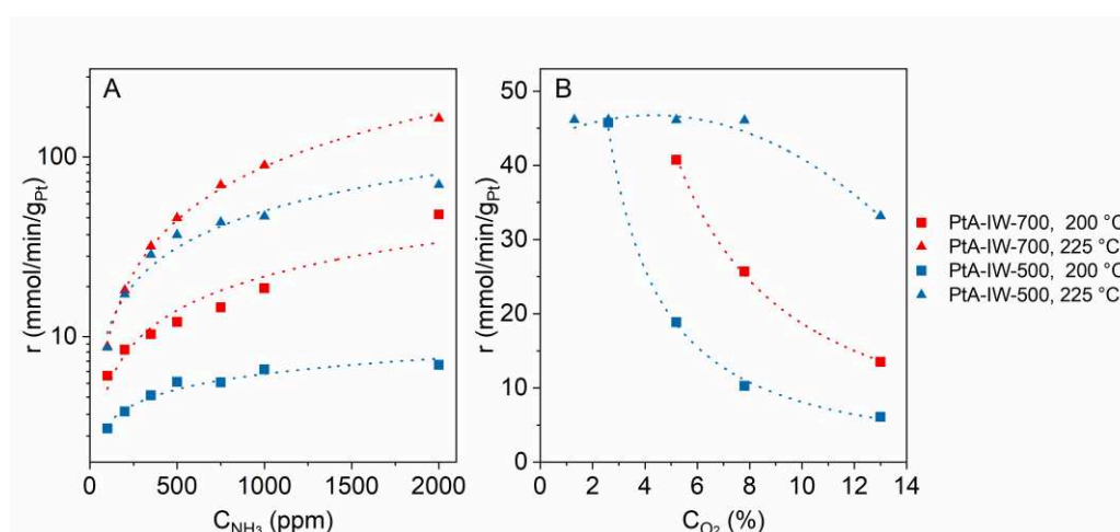
Figure 2. A – dependence of integral reaction rate on NH 3 concentration (constant O 2 concentration of 13 %); B – dependence of integral reaction rate on O 2 concentration (constant NH 3 concentration of 500 ppm). Catalysts: PtA-IW-700, PtA-IW-500.
