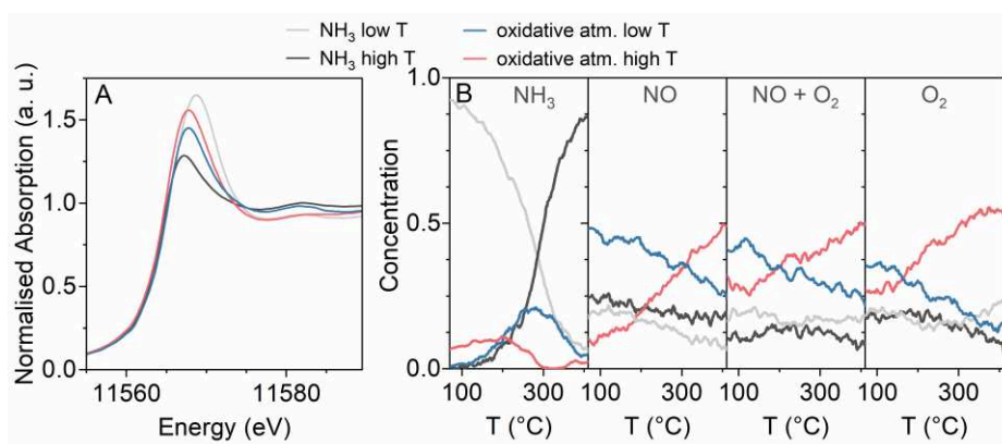
Figure 9. A – MCR-derived most distinct spectral components for the Pt L_3 XANES spectra recorded during heating of PtA-IW-500 in reductive ( \text{NH}_3 ) and oxidative ( \text{NO} , \text{O}_2 , and their mixture) atmospheres. B – contributions of the four most distinct MCR-derived spectral shapes to the experimental spectra during heating in reductive and oxidative atmospheres. For the spectral components in all atmospheres presented in the figure, low temperature and high temperature correspond to 50 and 400 °C, respectively.
