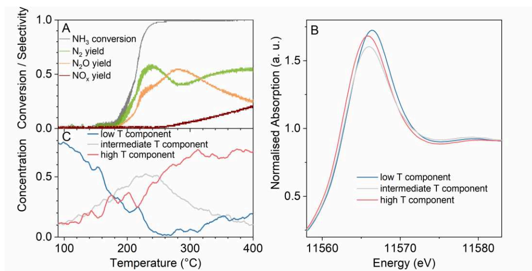
Figure 7. Results of operando QEXAFS measurements for PtA-IW-500 during the second heating in the reaction mixture (500 ppm NH 3 and 10 % O 2 , inert balance): A – catalytic data; B – the most distinct spectral components derived by MCR; C – contribution of the three most distinct spectral components to the experimental spectra. Maximum concentrations for spectral components were observed at the following temperatures: low-temperature component – below 100 °C; intermediate-temperature component – about 230 °C; high-temperature component – above 310 °C.
