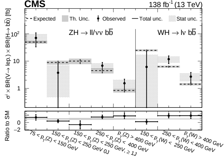
Figure 8: Measured values of \sigma \mathcal{B} , defined as the product of the VH production cross sections multiplied by the branching fractions of V \rightarrow \text{leptons} and H \rightarrow b\bar{b} , evaluated in the same STXS bins as for the signal strengths, combining all years. In the lower panel, the ratio of the observed results, with associated uncertainties, to the SM expectations is shown. If the observed signal strength for a given STXS bin is negative, no value is plotted for \sigma \mathcal{B} in the upper panel.
