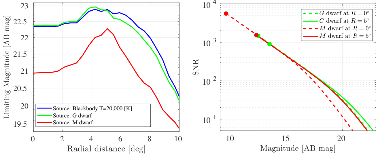
Figure 6. Left: Limiting point source AB magnitude achieved in 3 \times 300 s ULTRASAT exposures, plotted as a function of radial distance from the field center. Right: ULTRASAT’s Signal-to-Noise Ratio (SNR) as a function of AB magnitude for 3 \times 300 s exposures, for G and M dwarfs at the FoV center and at R = 5^\circ . The dots at the end of each curve mark the saturation limit.
