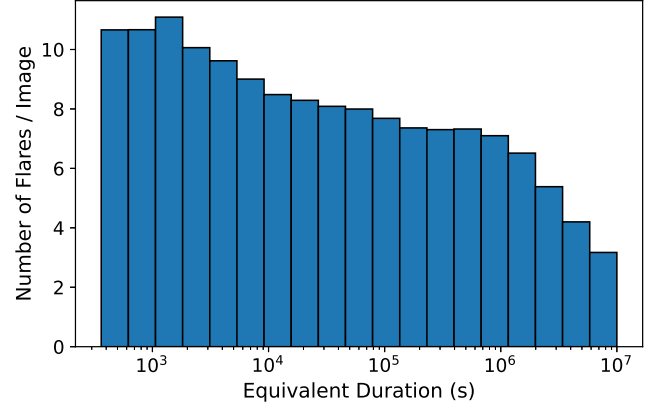
Figure 9. The expected distribution of flares detected in each 300s ULTRASAT image, for the dM population shown in Figure 8. The high energy tail of the distribution, with equivalent duration \geq 10^4 s, is poorly constrained. A Monte-Carlo simulation in which the NUV FFD was empirically derived from GALEX observations suggests each ULTRASAT image will capture \sim 150 flares from dM stars (Rekhi et al. 2023, submitted).
