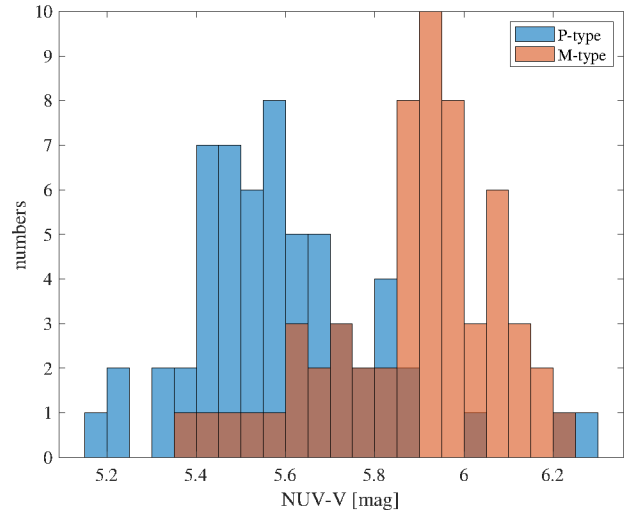
Figure 15. Distribution of NUV-V colors of P- (bluish) and M-type (reddish) asteroids measured by the GALEX space telescope (Waszczak et al. 2015). The Vmag is from the Minor Planet Center (MPC). Mean values are separated by about 0.3 mag, a value which is larger value than ULTRASAT photometric precision.
