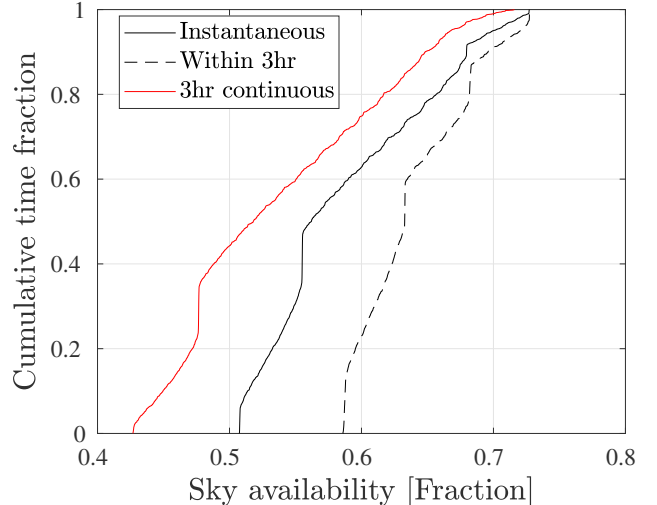
Figure 3. Sky availability for ToO observations under ULTRASAT pointing restrictions. At any given time ULTRASAT can access > 50\% of the sky, and > 58\% within 3 hrs. The minimal sky fraction for a 3-hr continuous observation (the nominal ToO duration) is 42\% , and the median is 51\% .
