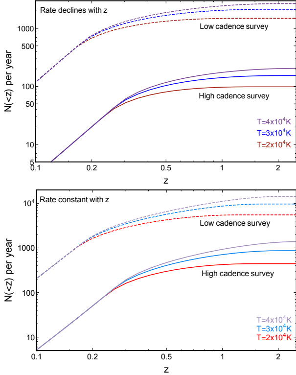
Figure 11. The cumulative number of TDEs detected per year within a given redshift, N(<z) . Colors show the effective blackbody temperatures T of TDE spectra at peak; we consider the idealized cases of T = 2 \times 10^4 K (red), T = 3 \times 10^4 K (blue), T = 4 \times 10^4 K (purple). Detection rates are shown assuming a volumetric rate that declines steeply with z (top panel, dark colors) or one that is constant with z (bottom panel, light colors). In this rate calculation, we consider both the high-cadence (solid lines) and low-cadence (dashed lines) survey modes. In the low-cadence calculations, we count as a “detection” every TDE with a peak magnitude m \leq 22.5 , while in the high-cadence calculations, we assume faint exposures over the course of one day are co-added up to a confusion limit of m = 23.5 .
