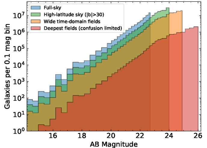
Figure 13. Expected number-magnitude distribution for galaxies in ULTRASAT surveys. Different colors represent different tiers of ULTRASAT survey. The all-sky survey is subdivided into the high latitude portion (green) and the shallower observations over the full sky including low galactic latitudes (blue). The time domain fields are similarly divided into the low-cadence, wide area portion (yellow) and the deepest fields (red). Each colored histogram is cut off at the magnitude limit appropriate to that survey’s anticipated integration time and the 10–11'' PSF expected over most of the field, except for the deep field histogram, which terminates at the 5\sigma confusion limit for a 6'' PSF. See text for discussion of samples upon which the plot is based.
