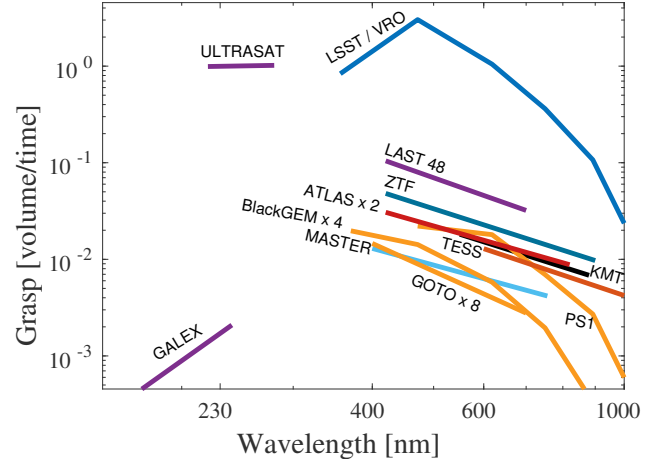
Figure 1. The volume of the universe per unit time (grasp; Ofek & Ben-Ami 2020a) accessible to several past, current and future sky surveys (VRO/LSST, Ivezić et al. 2019; LAST, Ofek et al. in prep.; ZTF, Bellm et al. 2019; ATLAS, Heinze et al. 2018; Pan-STARRS, Chambers et al. 2016; KMTNet, Kim et al. 2016; TESS, Ricker et al. 2015; BlackGEM, Bloemen et al. 2015; MASTER, Gorbovskoy et al. 2013; GOTO, Steeghs et al. 2022; GALEX, Martin et al. 2005), as a function of wavelength (normalized such that ULTRASAT’s grasp is 1). The grasp is given for a 20,000 K black-body source spectrum (e.g., a hot transient). ULTRASAT’s grasp is an order of magnitude larger than that of current surveys, two orders of magnitude larger than that of GALEX, the largest grasp UV mission to date, and comparable to that of LSST, the largest grasp optical survey under construction.
