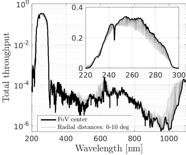
Figure 4. Left: ULTRASAT’s total throughput, accounting for all optical elements, the detector QE, and obscuration. The minor variation of the throughput across the field of view (gray curves) is due to the variation of the obscuration and of the angle-of-incidence distribution. Right: Color-color relation between ULTRASAT and Gaia -bands, for a range of main-sequence dwarfs (blue dots) and blackbody sources (red dots).
