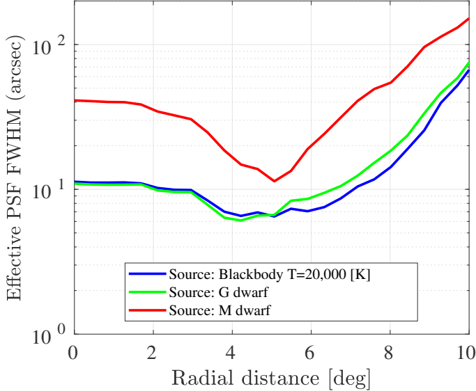
Figure 5. ULTRASAT’s radial-dependent effective PSF FWHM for three representative sources – G and M dwarfs, and a T = 20,000\text{K} blackbody source.
