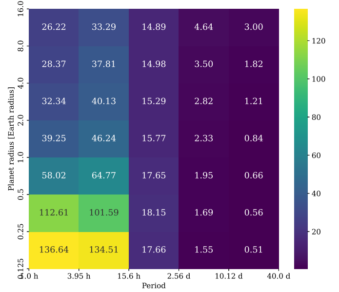
Figure 10. Maximum number of WD transiting planets detected by ULTRASAT, by both the low cadence survey and high cadence survey. Based on the current occurrence rate upper limits from van Sluijs & Van Eylen (2018).
