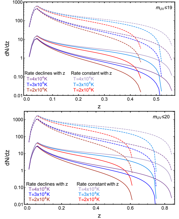
Figure 12. The differential number of TDEs suitable for spectroscopic followup detected per year around a certain redshift, dN/dz . Line styles and colors are the same as in Fig. 11, except that we now only count TDEs with peak UV magnitude m \leq 19 (top panel) or m \leq 20 (bottom panel). This restriction greatly reduces the maximum redshift out to which ULTRASAT will find TDEs of interest, and represents a factor of \sim 50 - 150 reduction from the total number of detected TDEs (for the m \leq 19 case).
