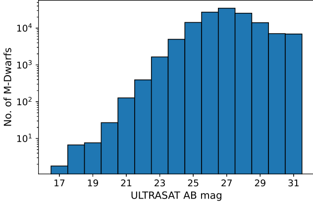
Figure 8. Magnitude distribution of dM stars in quiescence up to 800 pc in an exemplar ULTRASAT FoV of 200 \text{ deg}^2 . While flaring they can get up to \sim 5 mag brighter (Rekhi et al. 2023, submitted). Input catalogues used include the TESS Input Catalogue (Stassun 2019). Limiting magnitude for a 3 image co-add for dM stars is \approx 21.4 .
