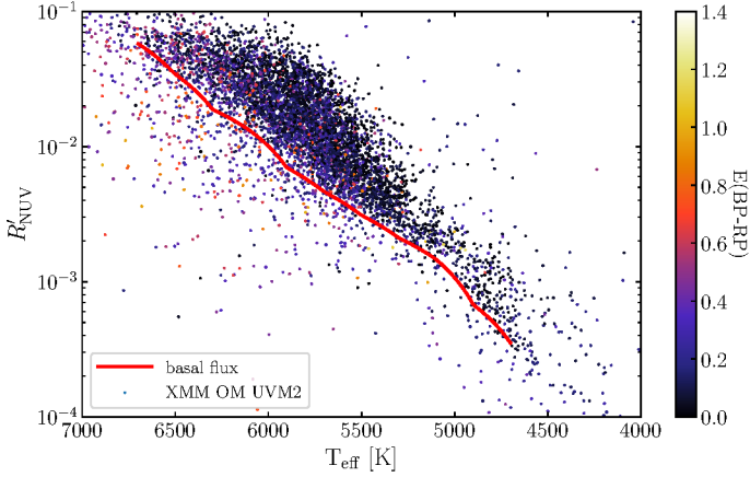
Figure 7. Relative chromospheric flux excess over the model photospheric flux, versus effective temperature, for 8859 stellar sources observed in the UV with the XMM-Newton Optical Monitor, in the Gaia DR2 source catalog, and in the LAMOST DR5 catalog. The color coding of the points reflects the reddening. The red line denotes the flux excess of the bottom 5th percentile of stars having reddening coefficient E(BP - RP) \leq 0.05 .
