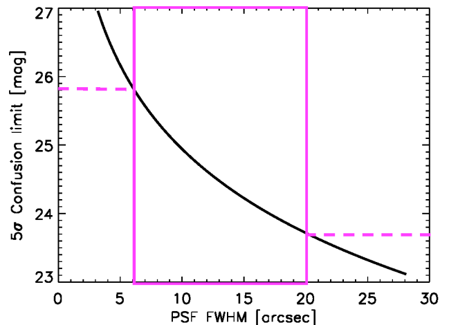
Figure 14. The 5\sigma confusion limit for near-UV imaging is plotted as a function of PSF size. The key range for ULTRASAT is approximately 6'' \leq \text{FWHM} \lesssim 20'' (cf. figure 5). Within its annulus of best focus ( 4^\circ < \theta < 6^\circ off axis), ULTRASAT can be used to study galaxies as faint as m_{AB} \approx 26 with integration times \sim 50 hours.
