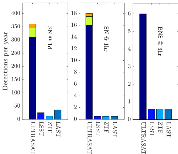
Figure 2. The number per year of supernova (SN) transients and EM transients following binary neutron star (BNS) mergers, expected to be detected at early time (as indicated in the plot) by ULTRASAT (assuming the limiting magnitude for 3 \times 300 \text{ s} exposures), the Vera Rubin Observatory (LSST), ZTF (Law et al. 2009) and LAST (Ofek & Ben-Ami 2020b). The blue/green/orange parts of the SN bars correspond to RSG/BSG/WR progenitors respectively. The SN rates are taken from Ganot et al. (2016), based on simulations calibrated to GALEX/PTF observations. The BNS rates were obtained assuming 12 GW detections per year out to 300Mpc, with UV flux similar to that observed following GW 170817.
