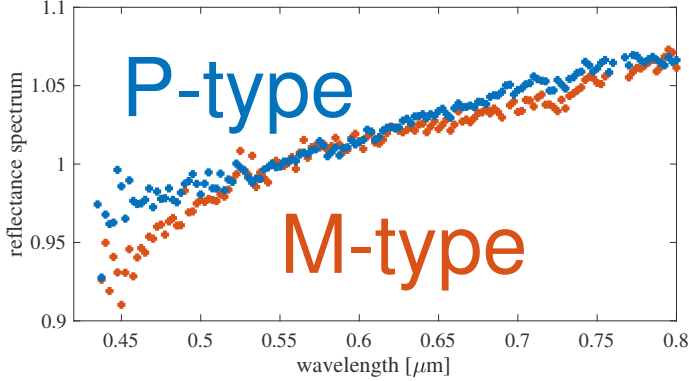
Figure 16. Visible reflectance spectra of asteroids 125 Libera (M-type, reddish) and 46 Hestia (P-type, bluish). Data from the SMASS library ( http://smass.mit.edu/ ), observation and classification conducted by Bus & Binzel 2002.
