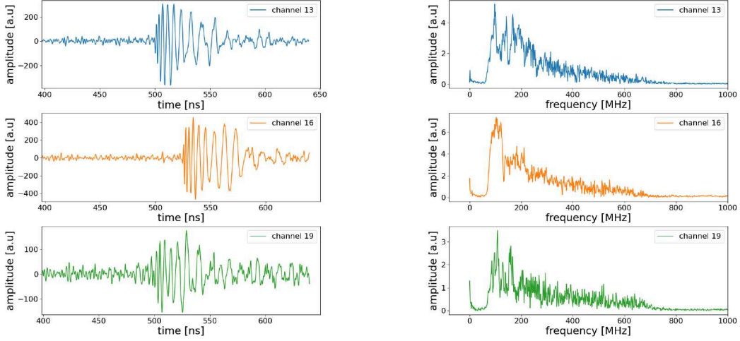
Figure 5: Voltage traces (left) and the frequency spectra (right) for the three upward facing channels (13, 16, 19) of the candidate event, Armstrong
