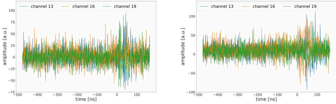
Figure 6: Voltage traces of the two candidate events with a low SNR for the three upward facing channels (13, 16, 19).
