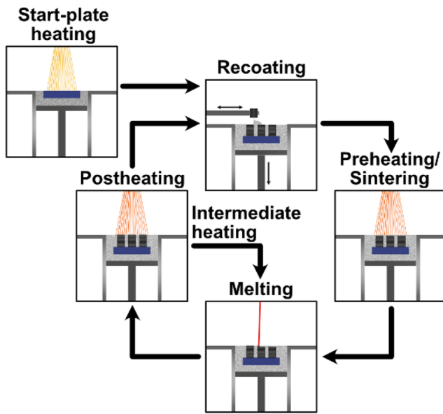
FIG. 1. Schematic of the typical process steps of the PBF-EB process. The start plate heating step is only used once at the beginning of the process, while the other steps are repeated for each layer until the build is finished.
