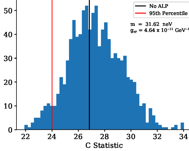
Figure 1: Histogram showing the likelihoods of the pseudo-random models of photon-ALP oscillation wiggles. This specific histogram shows our best case at a mass of 31.62 neV and a coupling of 4.64 \times 10^{-11} \text{ GeV}^{-1} .
