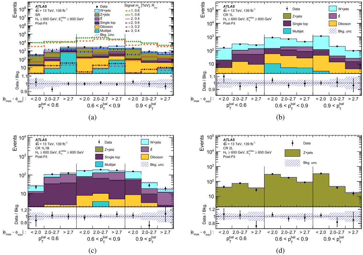
Fig. 3. The post-fit yields in the nine bins of the (p_T^{\text{bal}}, |\phi_{\text{max}} - \phi_{\text{min}}|) grid are shown for the (a) SR, (b) 1 L CR, (c) 1L1B CR, and (d) 2 L CR. Data are compared with background predictions, and six signal predictions covering a representative mediator mass and invisible fraction range are overlaid in the SR. Figure (a) shows a background-only fit in the SR. The uncertainties include all systematic and statistical components.
