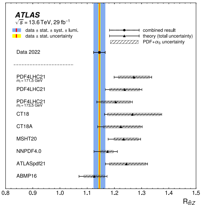
Fig. 4. Ratio of the t\bar{t} to the Z -boson cross section compared to the predictions for several sets of parton distribution functions. The total cross section for t\bar{t} production and the fiducial cross section for Z -boson production are used. If not explicitly mentioned, a top-quark mass of 172.5 GeV is assumed. The hatched box represents the PDF+ \alpha_s component of the uncertainty on the prediction. For the PDF4LHC21 PDF set, predictions for different assumptions about the top-quark mass are also displayed.
