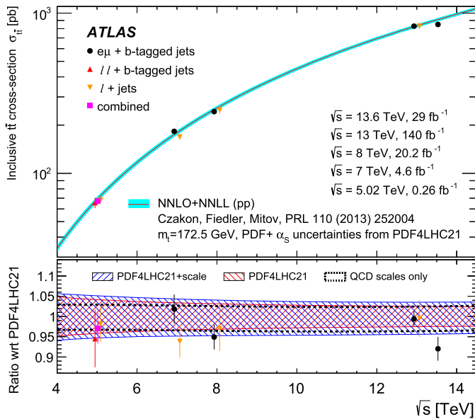
Fig. 3. Comparison of the measured t\bar{t} cross sections at various centre-of-mass energies and the theory predictions using the PDF4LHC21 PDF set. Measurements using the e\mu final state ( e\mu + b -tagged jets); ee , \mu\mu and e\mu final states ( \ell\ell + b -tagged jets); single lepton final states ( \ell + \text{jets} ); as well as combinations of final states (combined) are compared. The bottom panel shows the ratio of the measured values and three predictions that either contain only the uncertainties originating from the QCD scale variations (black), only the variations in the PDF uncertainties (red) or the total uncertainty in the prediction (blue).
