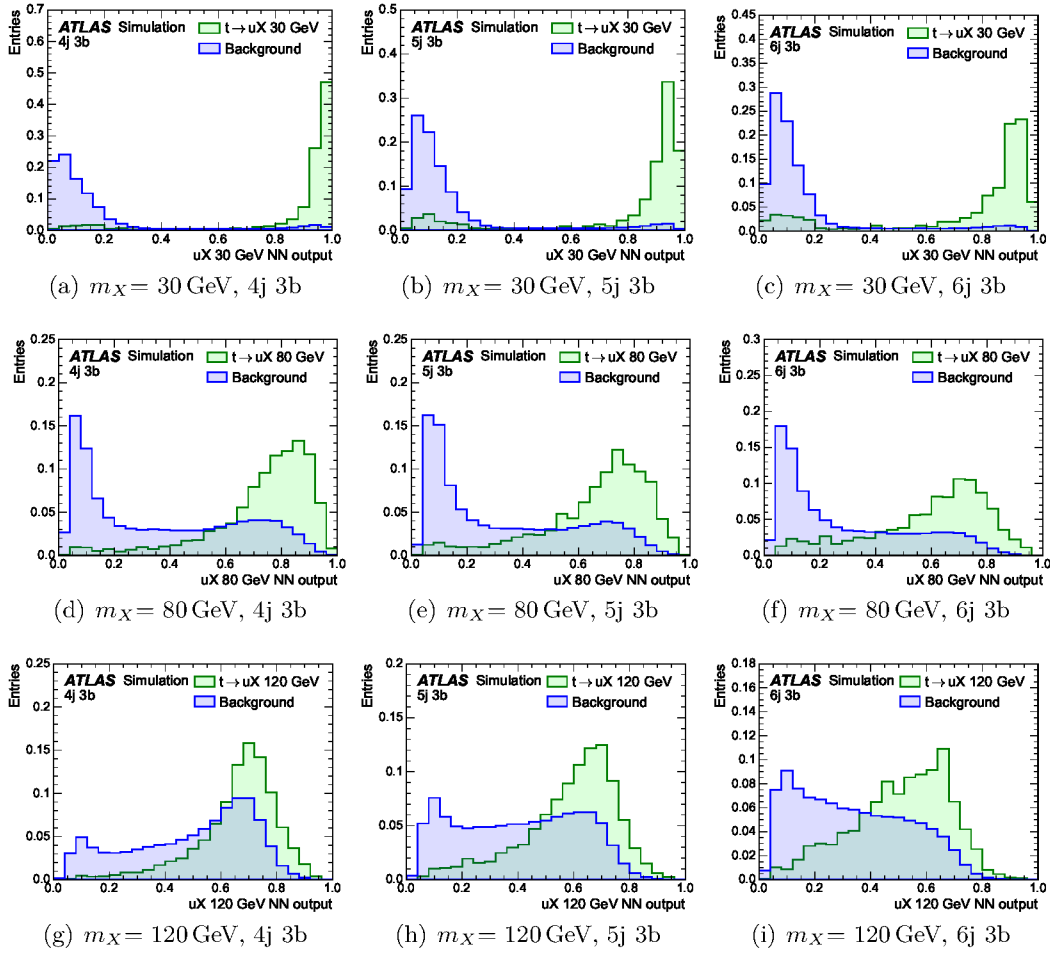
Figure 4. NN output distributions in the three signal regions for top-quark decays to uX under the 30, 80 and 120 GeV X mass hypotheses. Background samples are normalised according to their cross-sections. Signal and background distributions are finally normalised to the same area.
