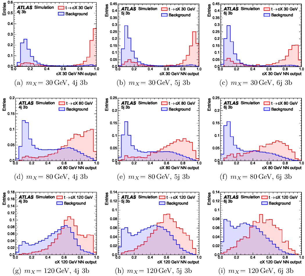
Figure 5. NN output distributions in the three signal regions for top-quark decays to cX under the 30, 80 and 120 GeV X mass hypotheses. Background samples are normalised according to their cross-sections. Signal and background distributions are finally normalised to the same area.
