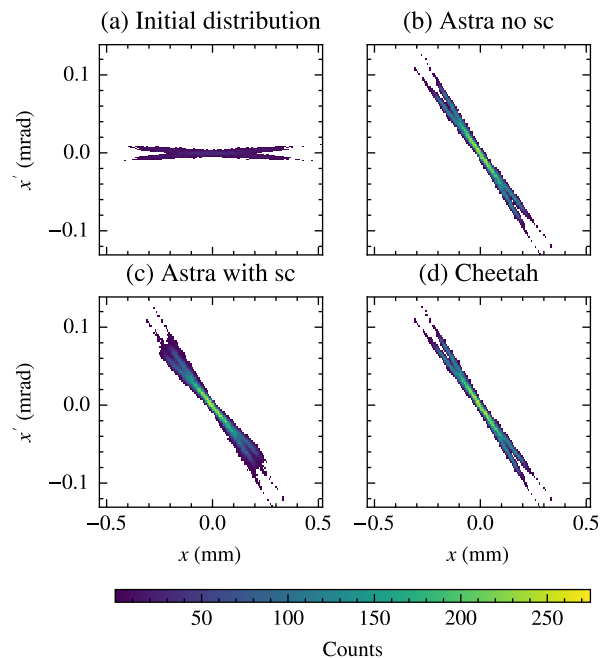
FIG. 10. Transverse phase spaces of a 5 pC beam in (x, x') plane through the ARES EA section. (a) Initial distribution of the beam with an arbitrary non-Gaussian shape. (b) Output distribution using ASTRA tracking without space charge effect. (c) Output distribution using ASTRA tracking with space charge effect. (d) Output distribution using Cheetah tracking.
