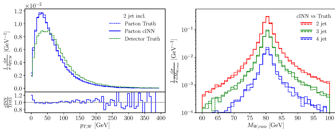
Figure 12: Unfolded parton-level distributions for the process pp \rightarrow Z_{\ell\ell} W_{jj} + \text{jets} using a cINN. The unfolding covers detector effects as well as additional jet radiation. Figure from Ref. [95].
