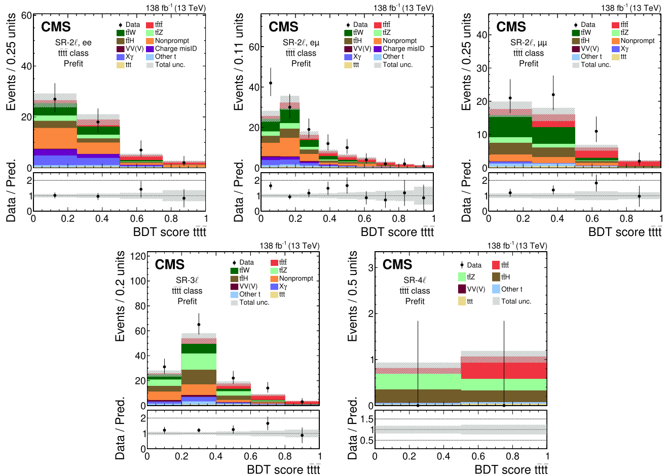
Fig. A.4. Comparison of the number of observed (points) and predicted (colored histograms) events in the BDT score t\bar{t}\bar{t} in the t\bar{t}\bar{t} classes of SR-2 \ell , shown for the ee (upper left), e\mu (upper middle), and \mu\mu (upper right) categories, of SR-3 \ell (lower left) and of SR-4 \ell (lower right). The vertical bars on the points represent the statistical uncertainties in the data, and the hatched bands the total uncertainty in the predictions. The signal and background yields are shown before the fit to the data (“prefit”).
