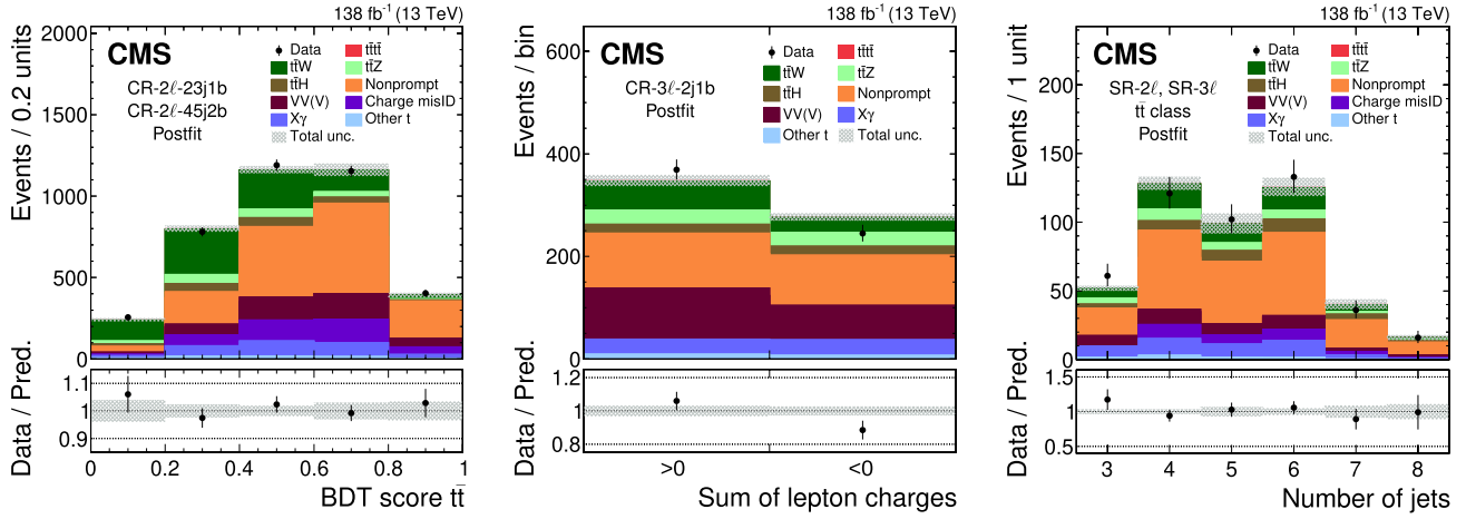
Fig. 6. Comparison of the number of observed (points) and predicted (colored histograms) events in the BDT score t_{\bar{t}} in the combined CR-2 \ell -23j1b and CR-2 \ell -45j2b (left), in the event yields with positive and negative sum of lepton charges in CR-3 \ell -2j1b (middle), and in the number of jets distribution in the t_{\bar{t}} class of the combined SR-2 \ell and SR-3 \ell (right). The vertical bars on the points represent the statistical uncertainties in the data, and the hatched bands the total uncertainty in the predictions. The signal and background yields are shown with their best fit normalizations from the simultaneous fit to the data (“postfit”).
