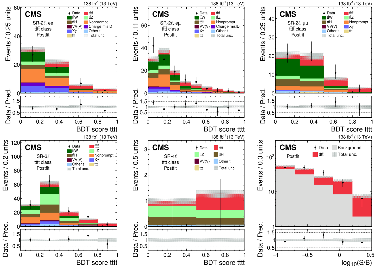
Fig. 7. Comparison of the number of observed (points) and predicted (colored histograms) events in the BDT score t\bar{t} in the t\bar{t} classes of SR- 2\ell , shown for the ee (upper left), e\mu (upper middle), and \mu\mu (upper right) categories, of SR- 3\ell (lower left) and of SR- 4\ell (lower middle). Additionally, the comparison is shown for all SRs combined as a function of \log_{10}(S/B) (lower right), where S and B are evaluated for each bin of the fitted distributions as the predicted signal and background yields before the fit to data. Bins with \log_{10}(S/B) < -1 are not included, and bins with \log_{10}(S/B) > 0.5 are included in the last bin. The vertical bars on the points represent the statistical uncertainties in the data, and the hatched bands the total uncertainty in the predictions. The signal and background yields are shown with their best fit normalizations from the simultaneous fit to the data (“postfit”).
