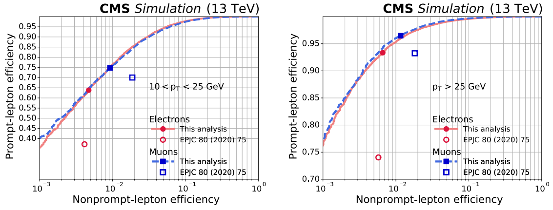
Fig. 2. Efficiency of selecting prompt leptons as a function of the misidentification probability for nonprompt leptons evaluated in simulated t\bar{t} events for the electron (red solid line) and muon (blue dashed line) ID BDT, shown for leptons with 10 < p_T < 25 GeV (left) and p_T > 25 GeV (right). Indicated with filled markers are the efficiencies for the ID criteria applied in this measurement and with empty markers those for the ID criteria applied in Ref. [41], where red circles and blue squares are used for electron and muon criteria, respectively.
