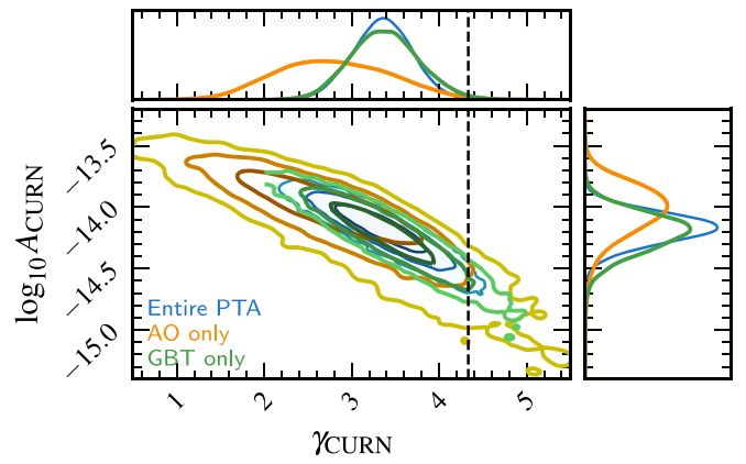
Figure 10. CURN ^\gamma posterior distributions for Arecibo (orange) and GBT (green) split-telescope data sets, and for the full data set (blue). The dashed line marks \gamma_{\text{CURN}} = 13/3 . The posteriors for the split-telescope data sets are consistent with each other and with the posteriors for the full data set.
