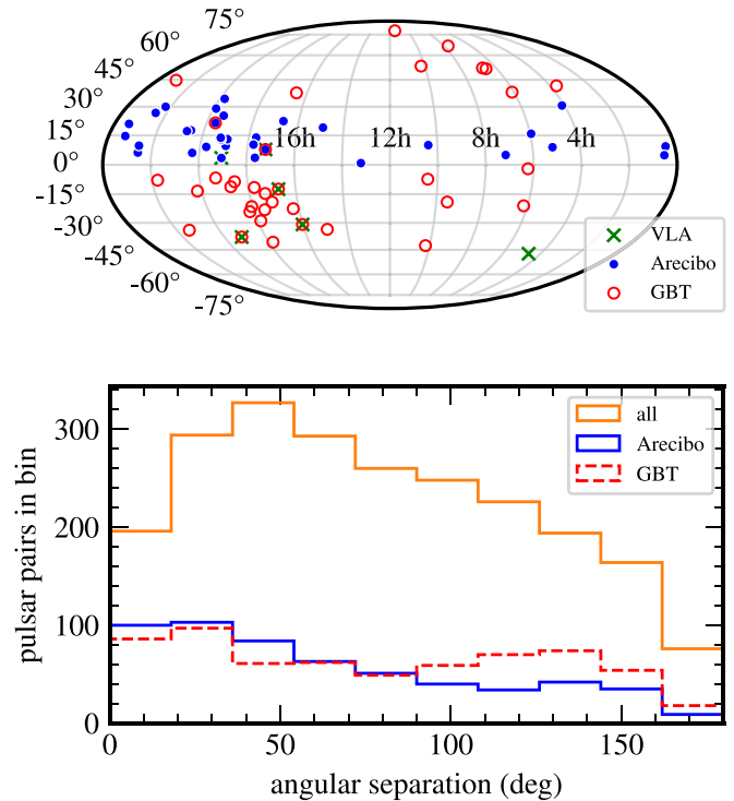
Figure 12. Top: sky locations of the 67 pulsars used in the 15 yr GWB analysis. Markers indicate which telescopes observed the pulsar. Bottom: distribution of angular separations probed by the pulsars in the full data set (orange), the Arecibo data set (blue), and the GBT data set (red). Because Arecibo and GBT mostly observed pulsars at different declinations, there are few intertelescope pairs at small angular separations, resulting in a deficit of pairs for the full data set in the first bin.
