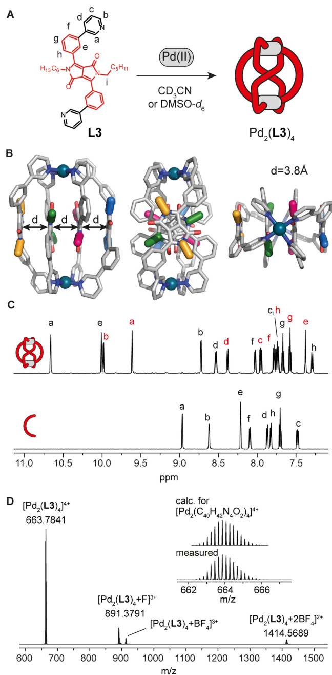
Figure 4. (A) Self-assembly of ligand L3 with 0.5 equiv. of Pd(II) cations to give [Pd 2 (L3) 4 ](BF 4 ) 4 . (B) Different views of the X-ray crystal structure of [Pd 2 (L3) 4 ](BF 4 ) 4 with the distances between the DPP backbones indicated. Alkyl chains and counterions are omitted for clarity. (C) Enlargement of the aromatic region of the 1 H NMR spectra in CD 3 CN of L3 and corresponding Pd-based assembly [Pd 2 (L3) 4 ](BF 4 ) 4 . (D) ESI-MS spectrum of [Pd 2 (L3) 4 + nBF 4 ] (4-n)+ with n = 0–2. The observed and calculated isotopic patterns of [Pd 2 (L3) 4 ] 4+ are shown in the inset.
