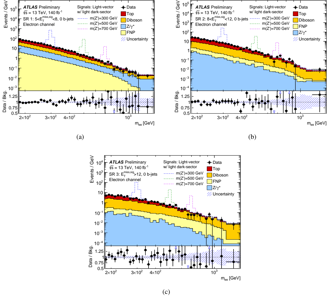
Figure 8: The m_{\ell\ell} distribution in the electron channel for SR 1 ( 5 < E_T^{\text{miss, sig}} < 8 ) (a), SR 2 ( 8 < E_T^{\text{miss, sig}} < 12 ) (b) and SR 3 ( E_T^{\text{miss, sig}} > 12 ) (c). The distributions are shown after performing a profile log-likelihood fit in the control and signal regions. The total uncertainty on the SM background is shown by the hatched band and it includes both statistical and systematic uncertainties. The last bin contains overflow events.
