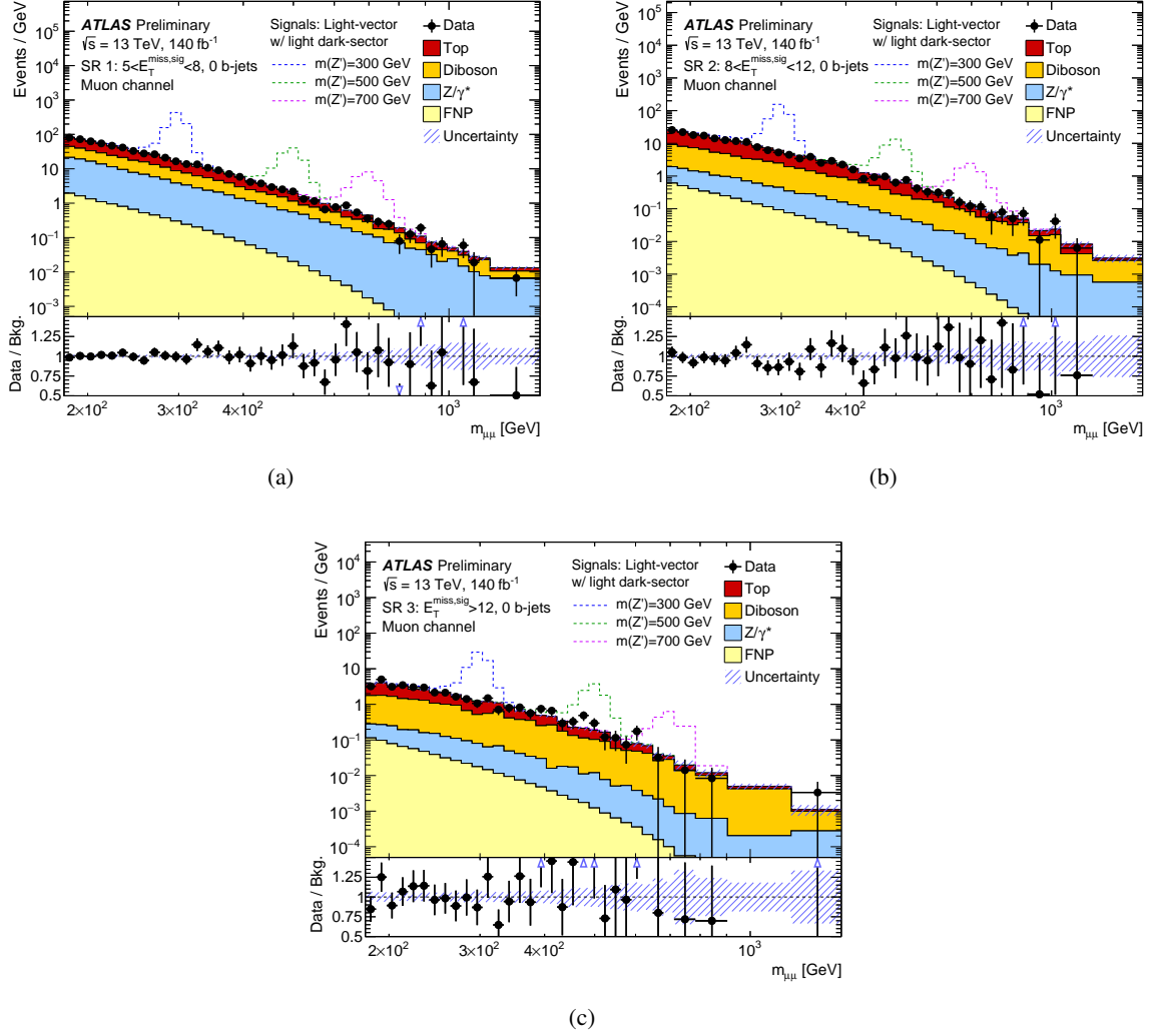
Figure 9: The m_{\ell\ell} distribution in the muon channel for SR 1 ( 5 < E_T^{\text{miss,sig}} < 8 ) (a), SR 2 ( 8 < E_T^{\text{miss,sig}} < 12 ) (b) and SR 3 ( E_T^{\text{miss,sig}} > 12 ) (c). The distributions are shown after performing a profile log-likelihood fit in the control and signal regions. The total uncertainty on the SM background is shown by the hatched band and it includes both statistical and systematic uncertainties. The last bin contains overflow events.
